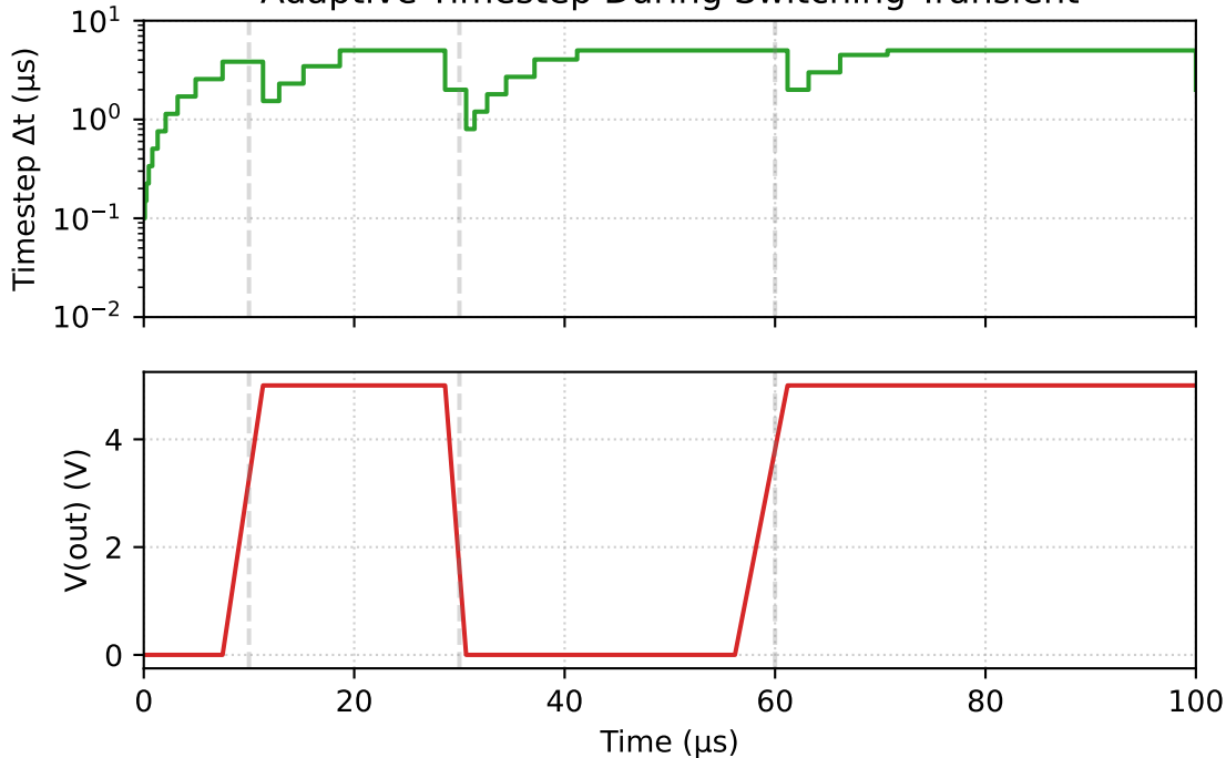
Adaptive Timestep During Switching Transient
