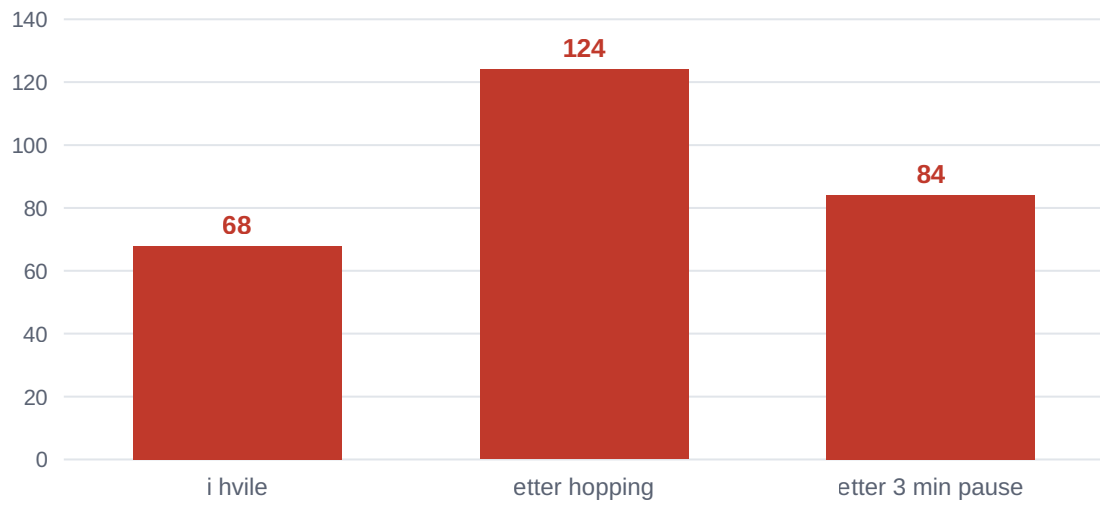
Figur 2.26 Aminas puls.
