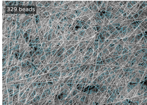
Otsu + watershed
