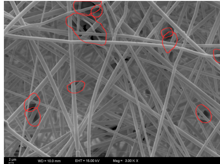
Z2-3 — 3000x — 10 beads
