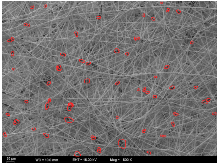
Z2-1 — 500x — 71 beads
