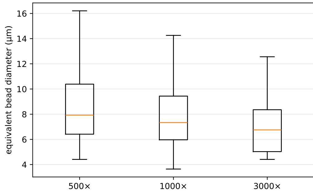
Physical bead size is stable across magnifications
