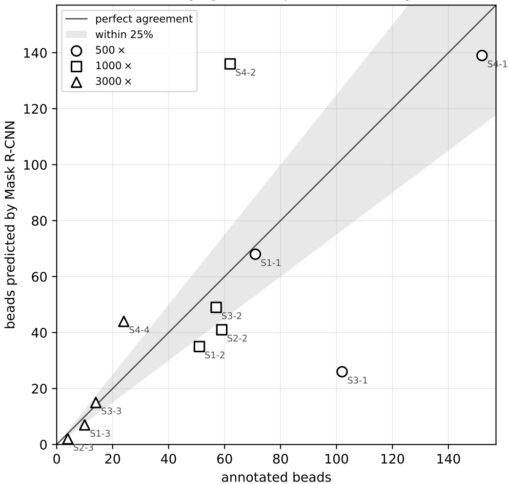
Counting agreement per held-out image
