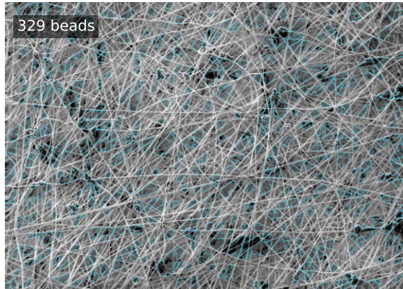
Otsu + watershed
