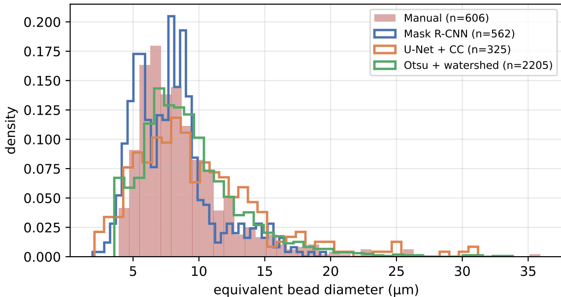
Predicted against manual bead size distribution, all held-out images
