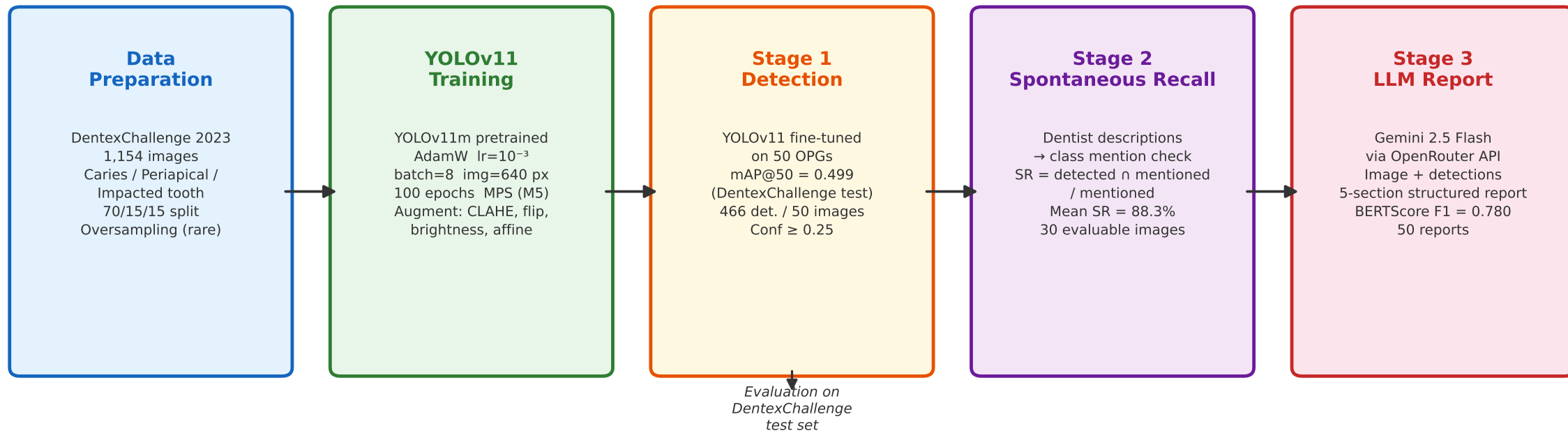
Fig. 1. Three-stage pipeline for panoramic dental radiograph analysis.
