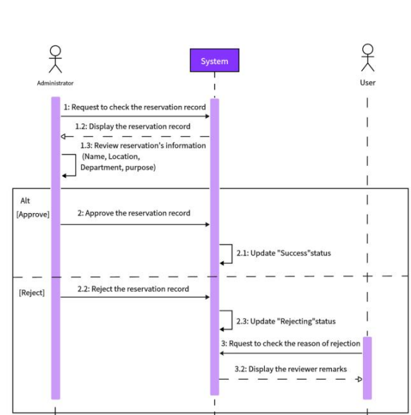
Figure 9 / APPENDIX 5: Administrator reviews meeting room booking records
