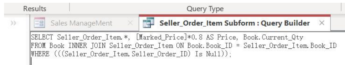
Figure28: Seller_Order_Item_Query
