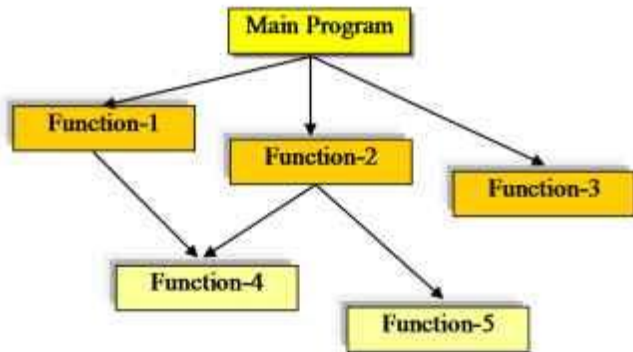
Procedure-oriented Programming
