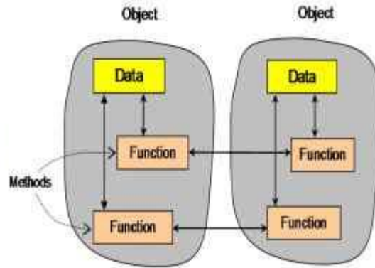
Object-oriented Programming
