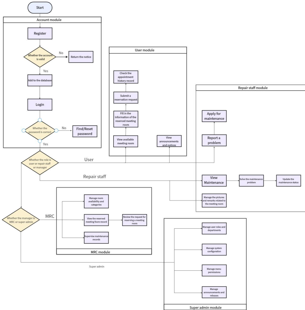
APPENDIX 6 - Figure 6 : Role login division flow chart
