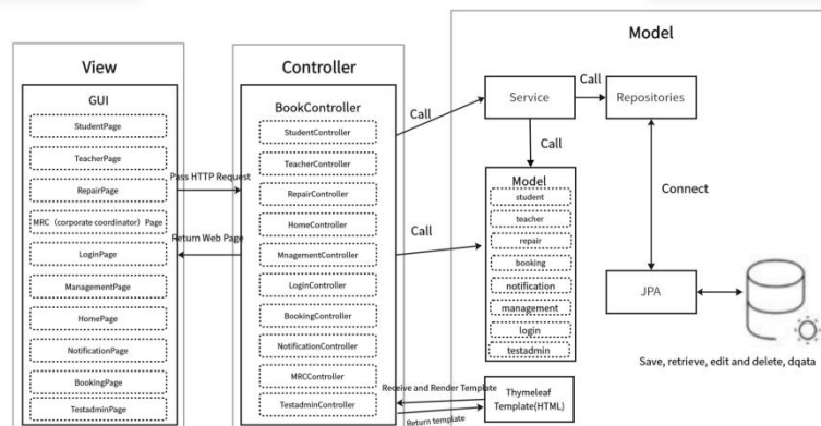
Figure 2 / APPENDIX 2 : MVC architecture
