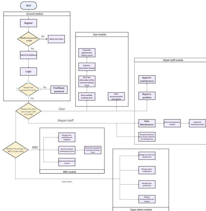
Figure 6 / APPENDIX 6 : Role login division flow chart
