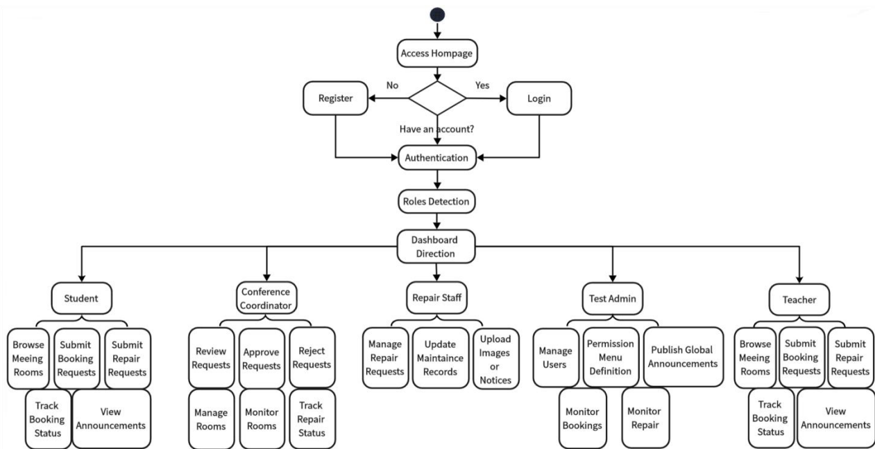
APPENDIX 5 - Figure 5 : Process Flow
