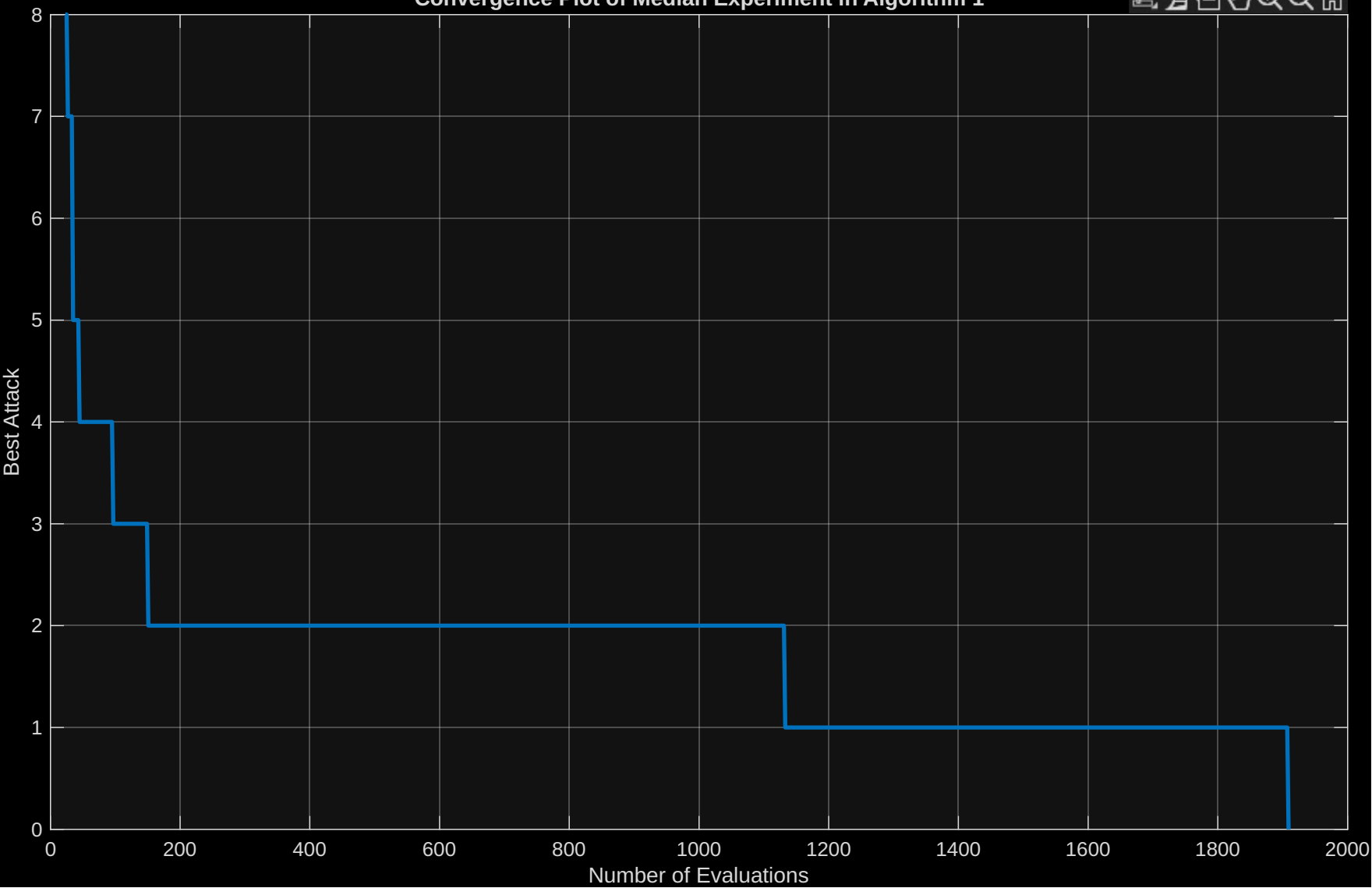
Convergence Plot of Median Experiment in Algorithm 1
