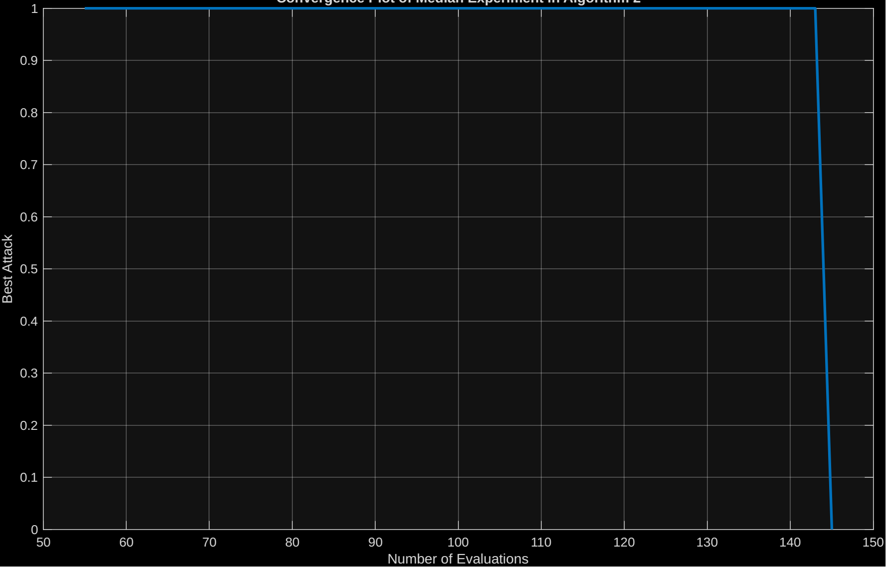
Convergence Plot of Median Experiment in Algorithm 2
