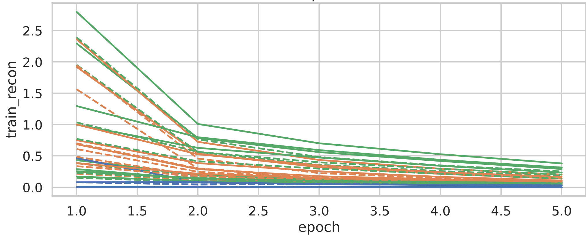
Strict Text-Koopman loss terms
