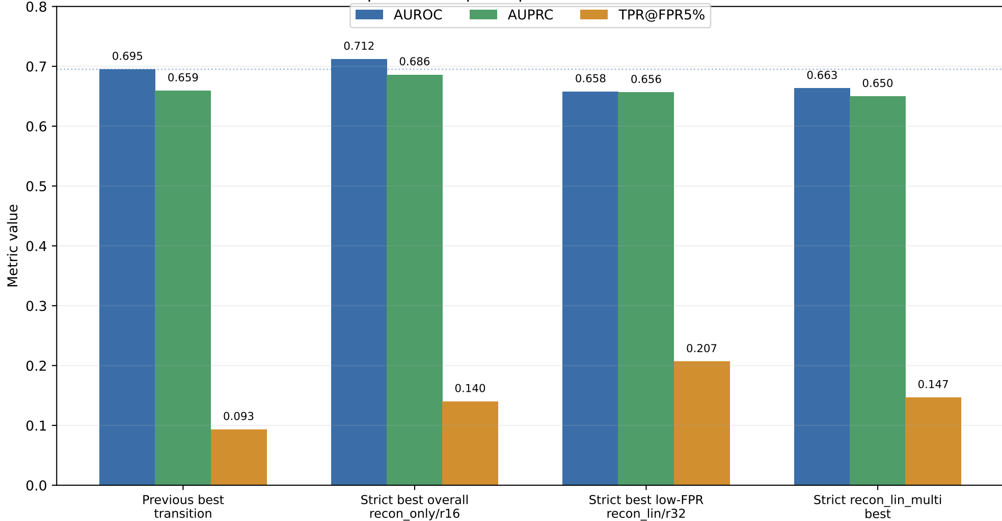
Strict Text-Koopman loss update produces a new best external result
