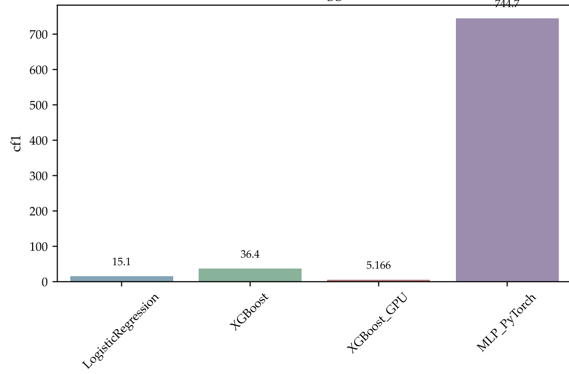
CF1: higgs
