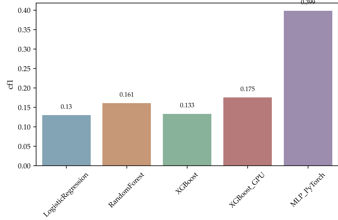
CF1: wine
