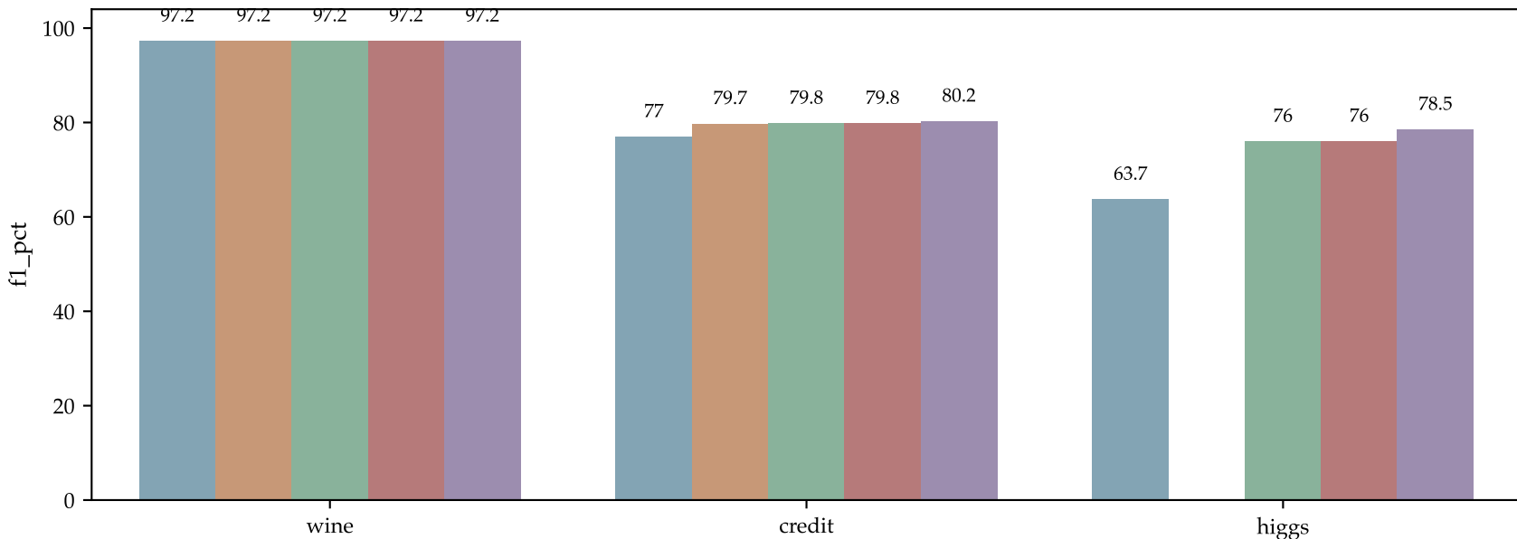
CF1: credit
