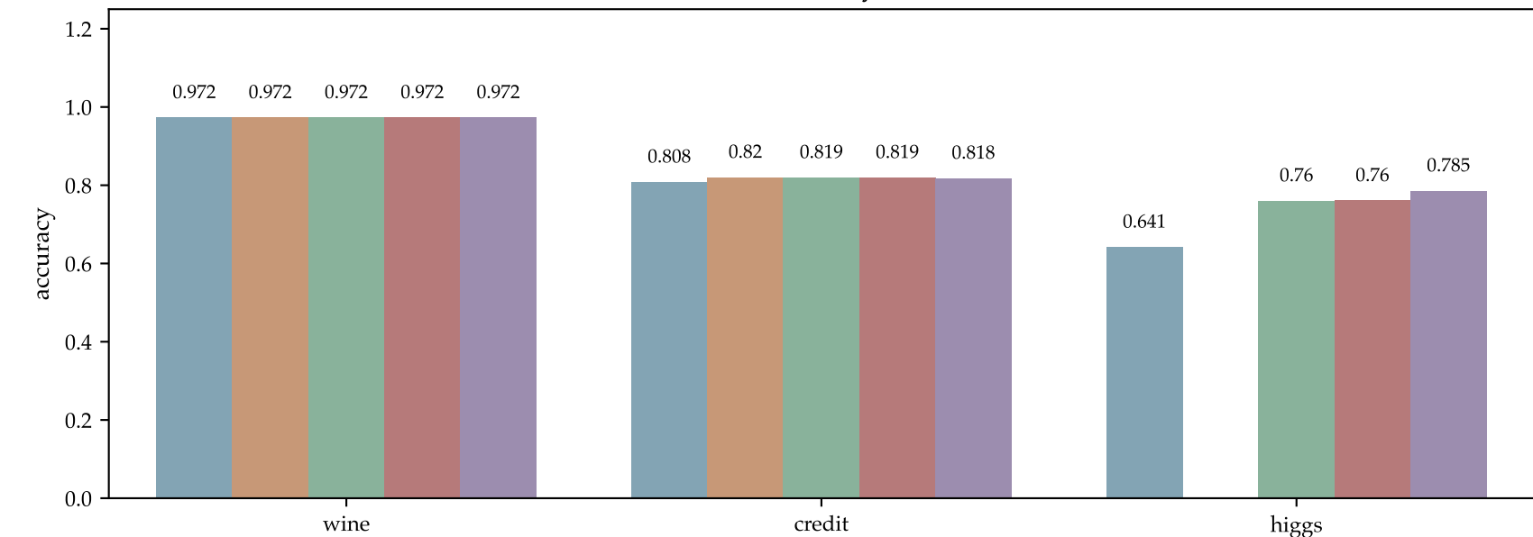
CF1: wine
