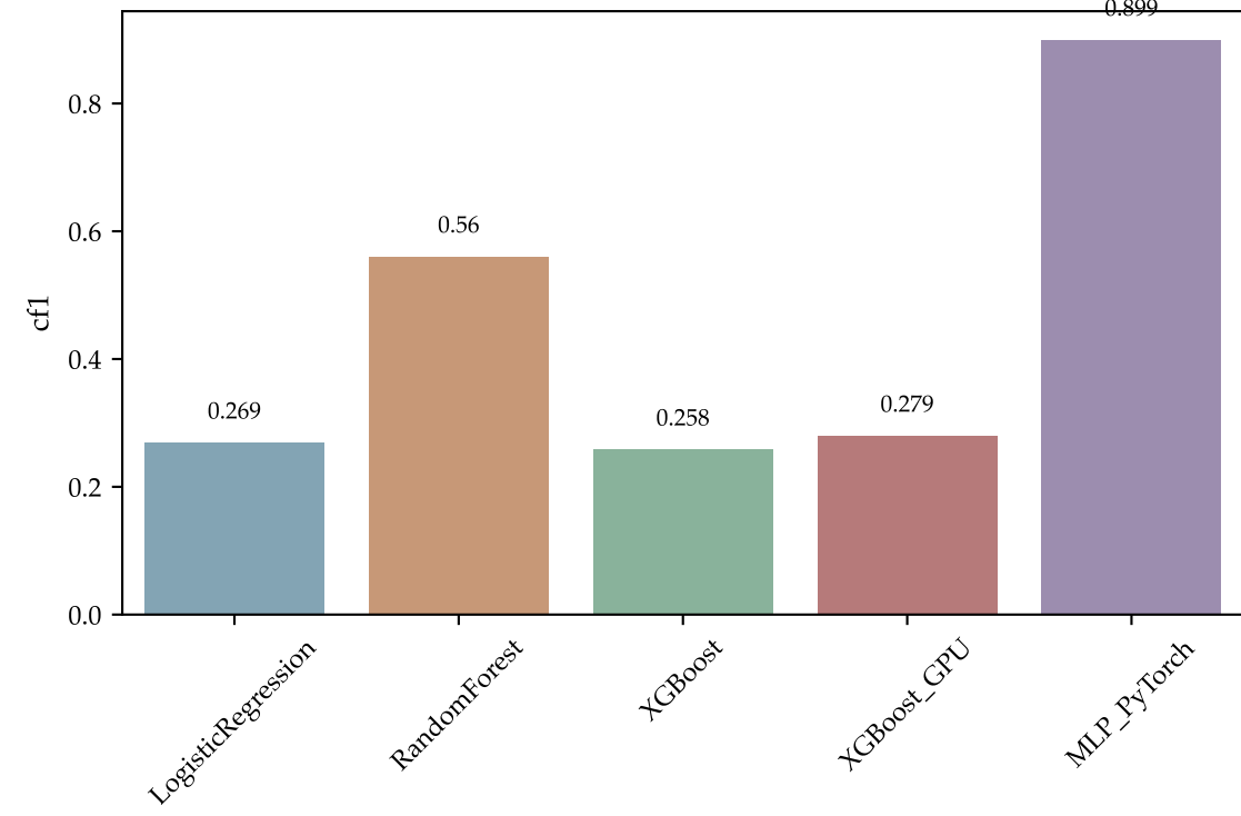
CF1: credit
