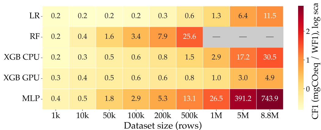
Figure 5.10: CF1 (mgCO 2 eq per WF1) for all model-size combinations. Colour encodes log-scaled CF1: yellow is most efficient, dark red is least. Cell annotations show raw CF1 values. Grey cells indicate runs not performed (RF excluded above 500,000 rows).
