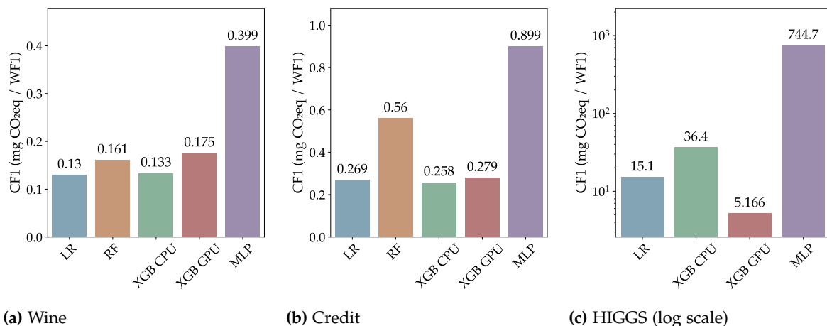
Figure 5.6: CF1 (mgCO 2 eq per WF1 percentage point) per model and dataset. Lower is better. The HIGGS panel uses a log scale. No single model leads across all three datasets.
