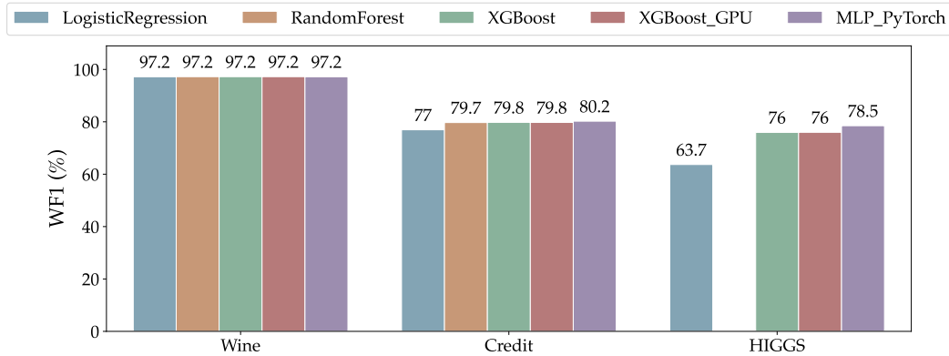
Figure 5.4: WF1 across all 14 model-dataset combinations. On Wine, all five models converge on a WF1 of 97.2%, making emissions the only meaningful dimension of comparison. On HIGGS, LR saturates well below the non-linear models and MLP achieves the highest single result in the study.
