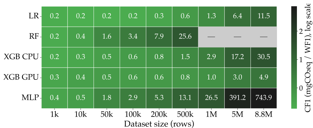
Figure 5.10: CF1 (mgCO 2 eq per WF1) for all model-size combinations. Colour encodes log-scaled CF1: green indicates the most efficient configurations, dark indicates the least. Cell annotations show raw CF1 values. Grey cells indicate runs not performed (RF excluded above 500,000 rows).
