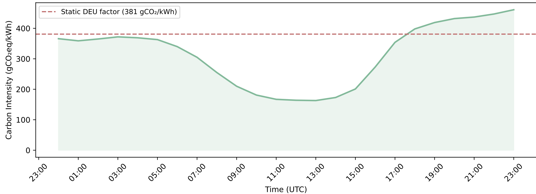
Hourly Carbon Intensity - Germany (DE) - Jul 24, 2024
