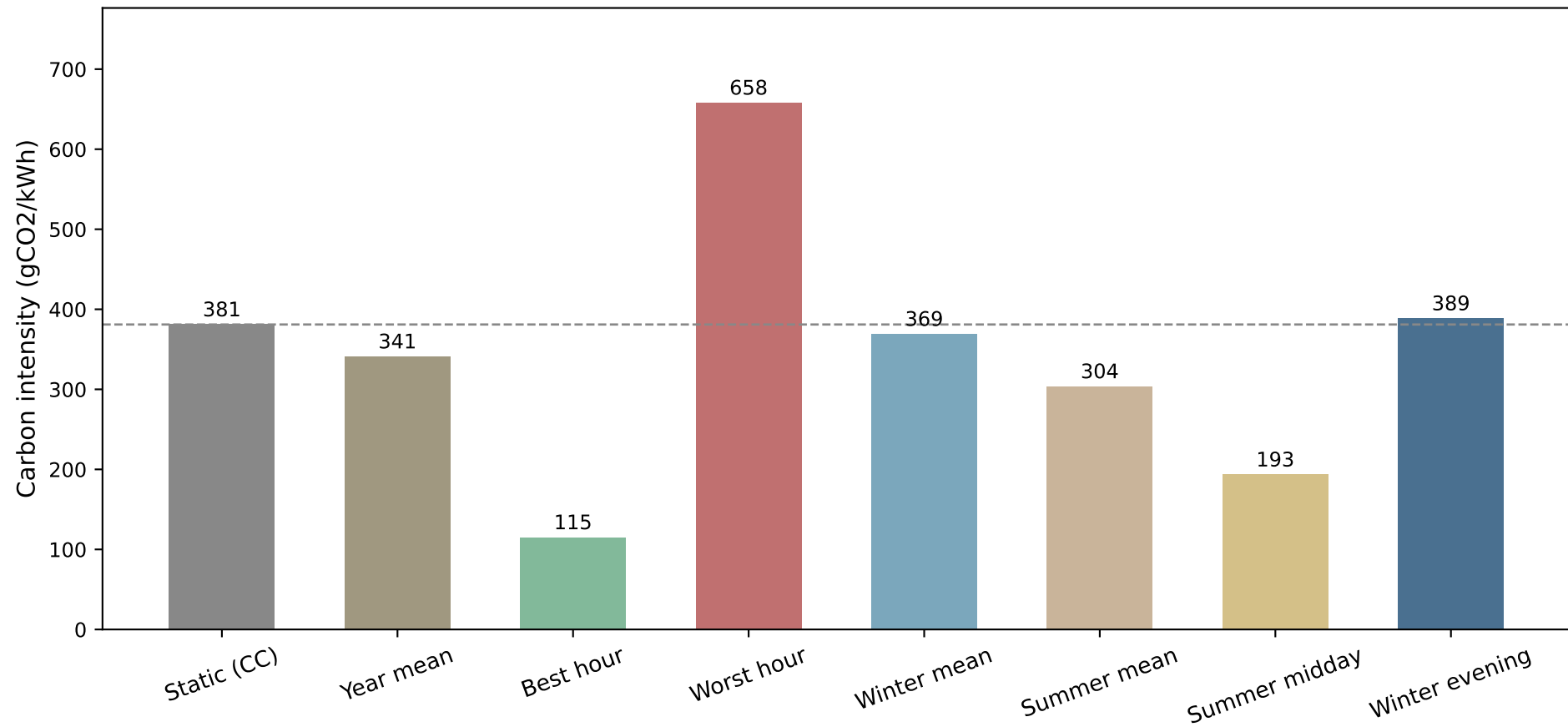
Grid carbon intensity per timing scenario — Germany 2024/2024
