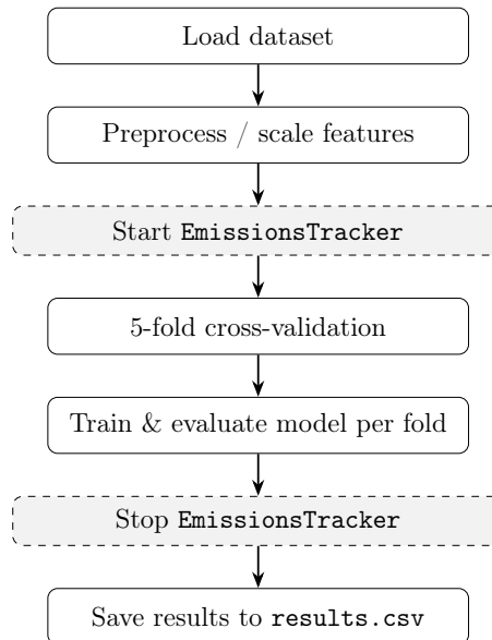
Figure 5.2: Training and emissions tracking procedure per model-dataset combination. Dashed boxes indicate CodeCarbon EmissionsTracker calls.
