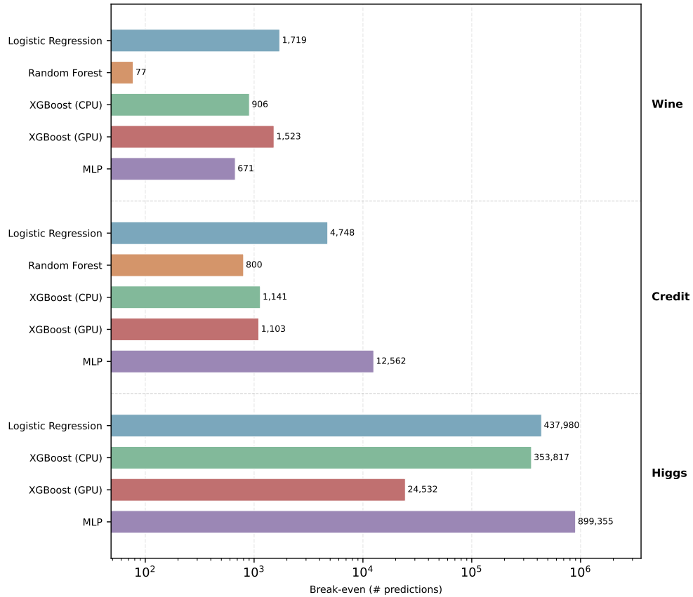
Figure 6.9: Break-even number of predictions at which cumulative inference CO 2 emissions surpass the one-time training footprint (log scale).
