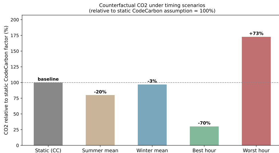
Figure 6.5: Counterfactual \text{CO}_2 relative to the static CodeCarbon baseline (= 100 %)
