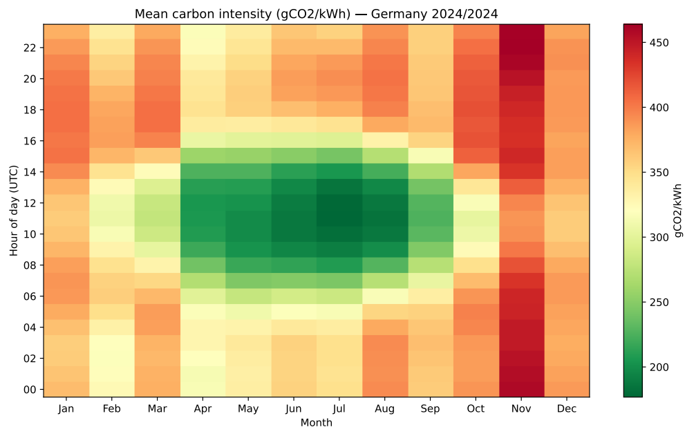
Figure 6.8: Mean carbon intensity (gCO 2 /kWh) by hour of day and calendar month for the German grid (2024), derived from 8,760 hourly observations.
