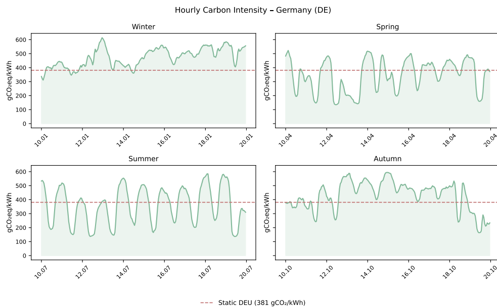
Figure 6.7: Hourly carbon intensity for representative ten-day windows per season, Germany 2025
