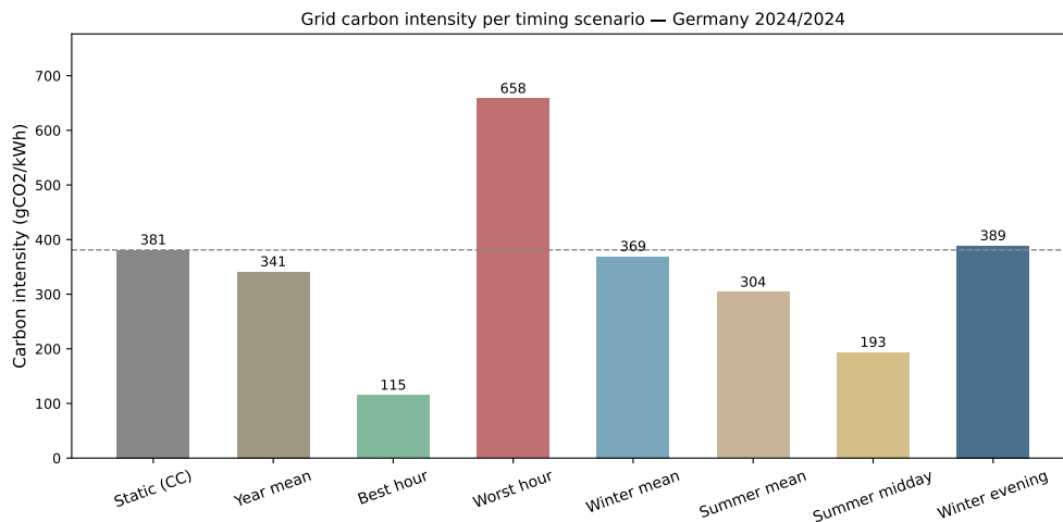
Figure 6.4: Carbon intensity (gCO 2 /kWh) for eight timing scenarios
