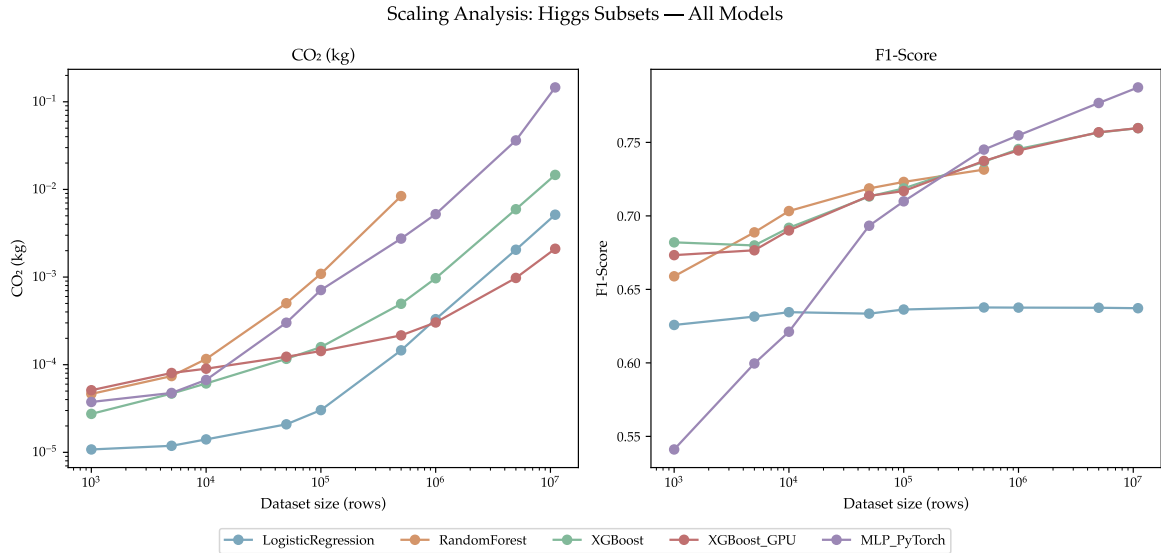
Figure 6.9: CO 2 emissions (log scale) and weighted F1-score across nine HIGGS subsets for all models. Random Forest excluded at full scale.
