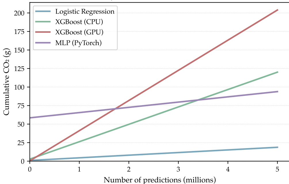
Lifecycle CO 2 : all models on HIGGS
