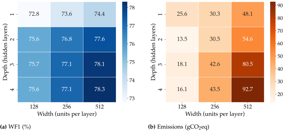
Figure 5.11: MLP architecture variation on HIGGS for all depth-width combinations. Left: WF1, where darker cells indicate higher WF1 (better). Right: training emissions in gCO 2 eq, where lighter cells indicate lower emissions (better).
