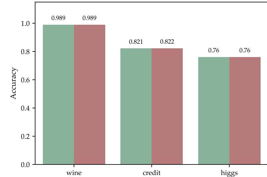
Accuracy
