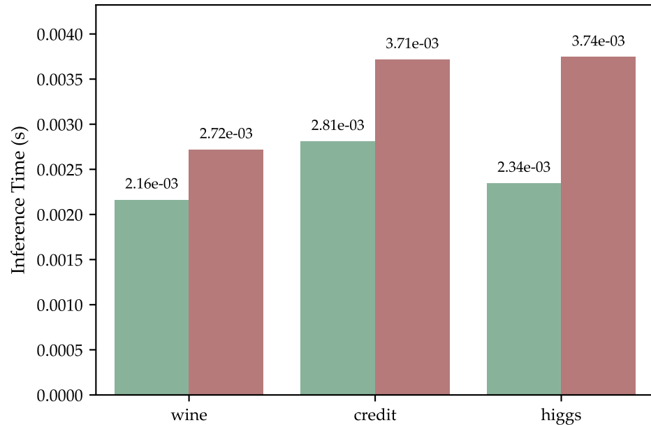
Inference Time
