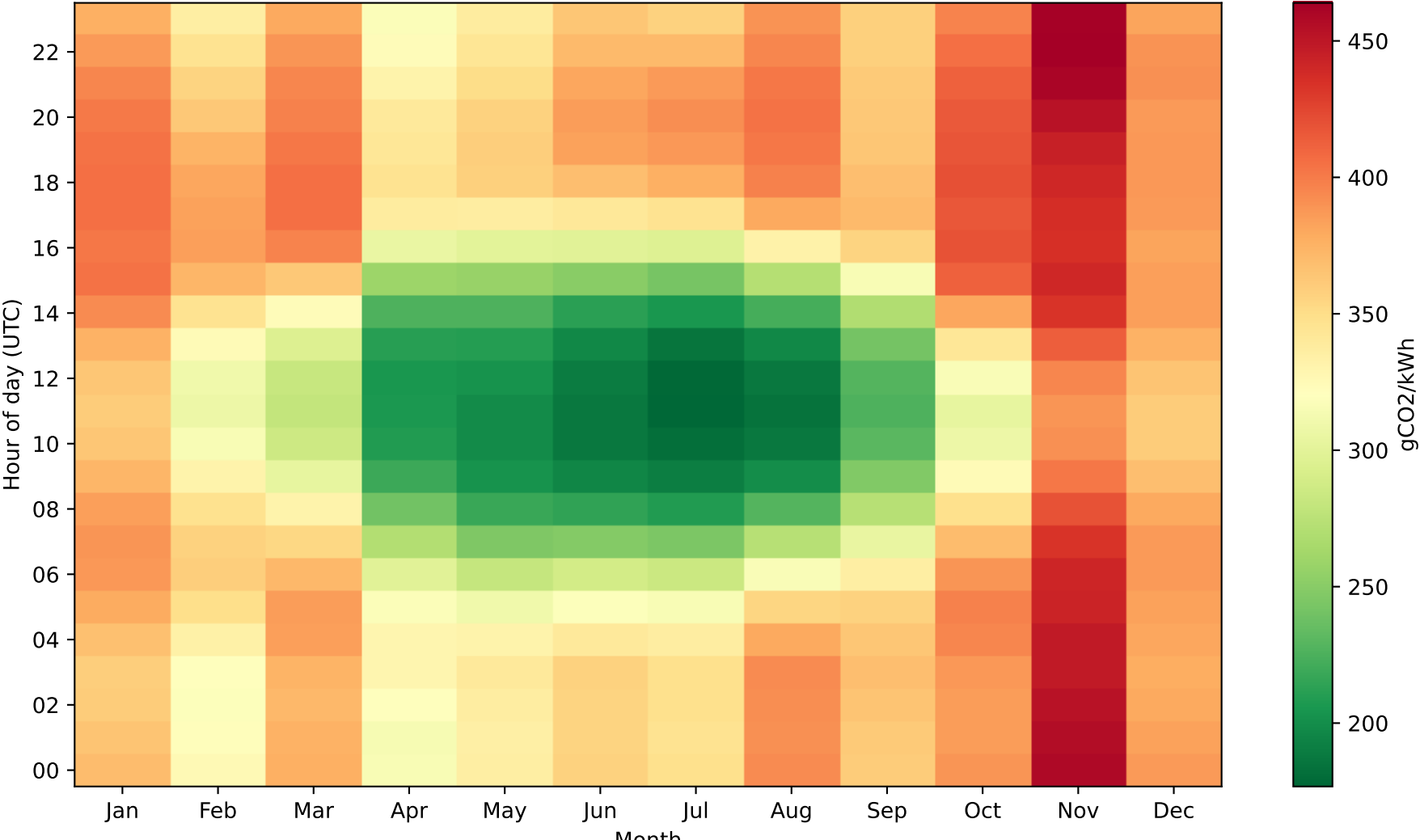
Mean carbon intensity (gCO2/kWh) — Germany 2024/2024
