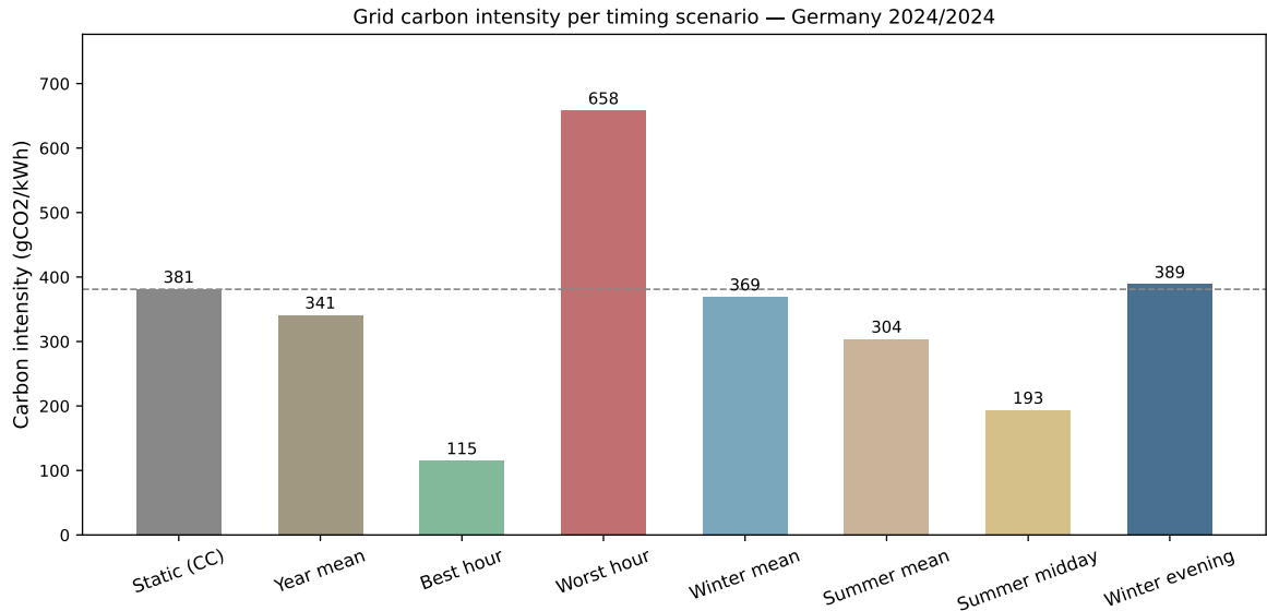
Figure 6.13: Carbon intensity ( \frac{\text{gCO}_2\text{eq}}{\text{kWh}} ) for eight timing scenarios
