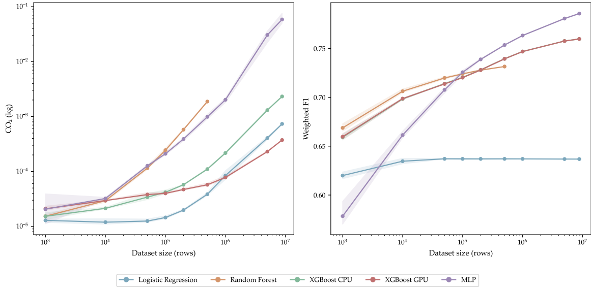
Figure 6.9: Emissions (log scale) and WF1 across nine HIGGS subsets for all models. Each point is the mean of three independent random-seed runs. RF excluded above 500,000 rows.
