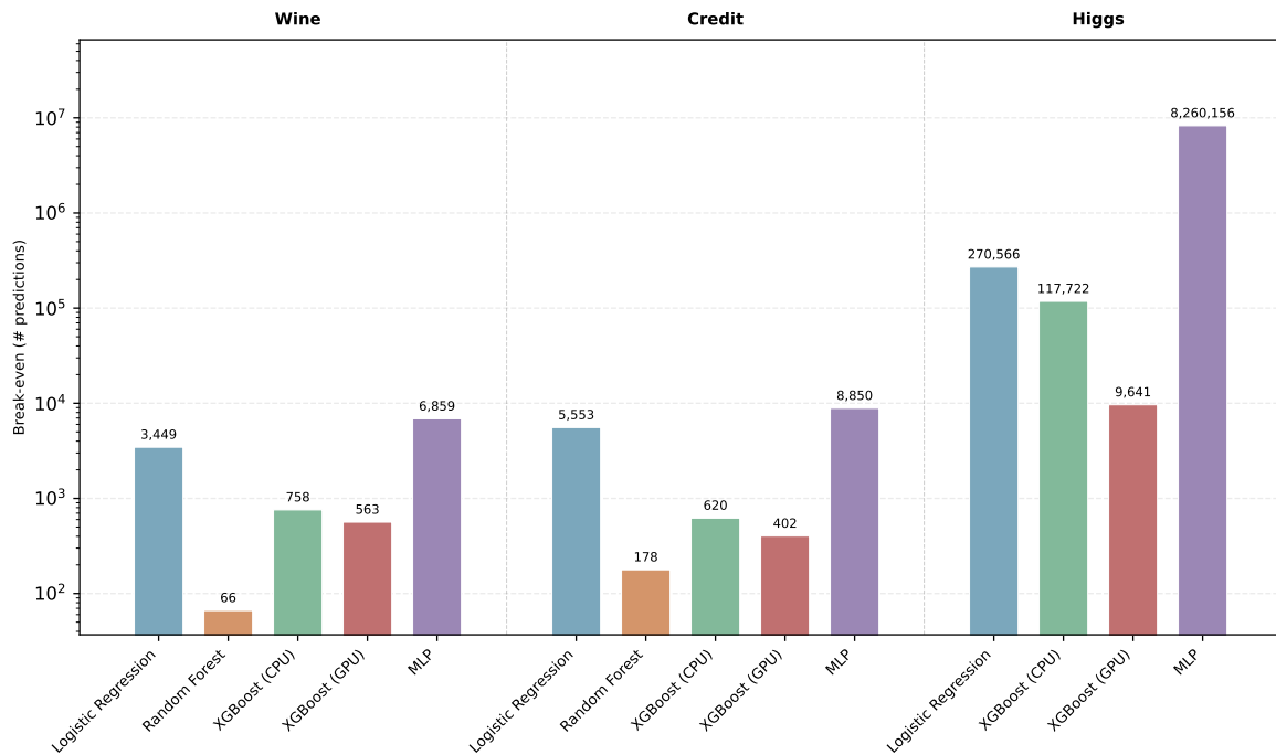
Figure 6.19: Break-even number of predictions at which cumulative inference emissions surpass the one-time training footprint (log scale).
