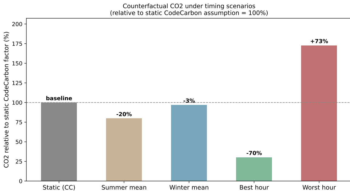
Figure 6.14: Counterfactual emissions relative to the static CodeCarbon baseline (= 100 %)
