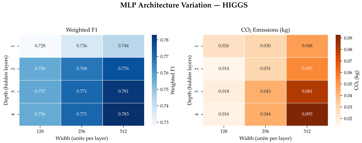
Figure 6.10: MLP architecture variation on HIGGS: WF1 (left) and emissions (right) for all depth-width combinations. Darker cells indicate higher values.
