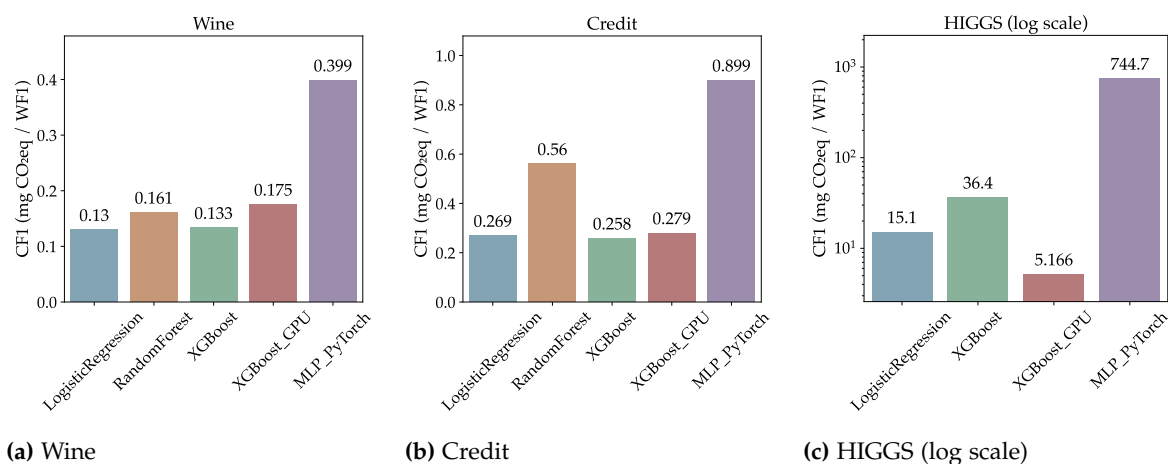
Figure 6.6: CF1 (mgCO 2 eq per WF1 percentage point) per model and dataset. Lower is better. The HIGGS panel uses a log scale. No single model leads across all three datasets.
