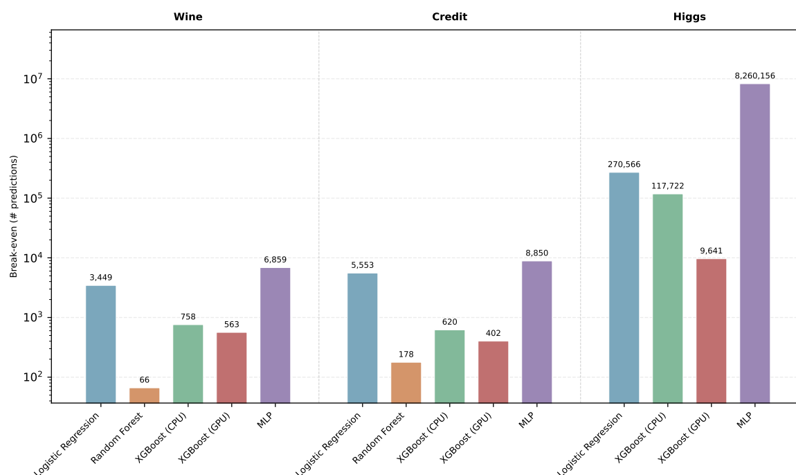
Figure 6.19: Break-even number of predictions at which cumulative inference CO 2 emissions surpass the one-time training footprint (log scale).
