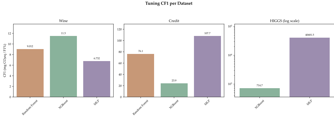
Figure 6.3: Tuning CF1 (mg CO 2 eq per WF1 percentage point) per tuning study, using the best WF1 across 40 trials as denominator. Lower is better. The HIGGS panel uses a log scale. Random Forest was not tuned on HIGGS. Literature defaults were used instead.
