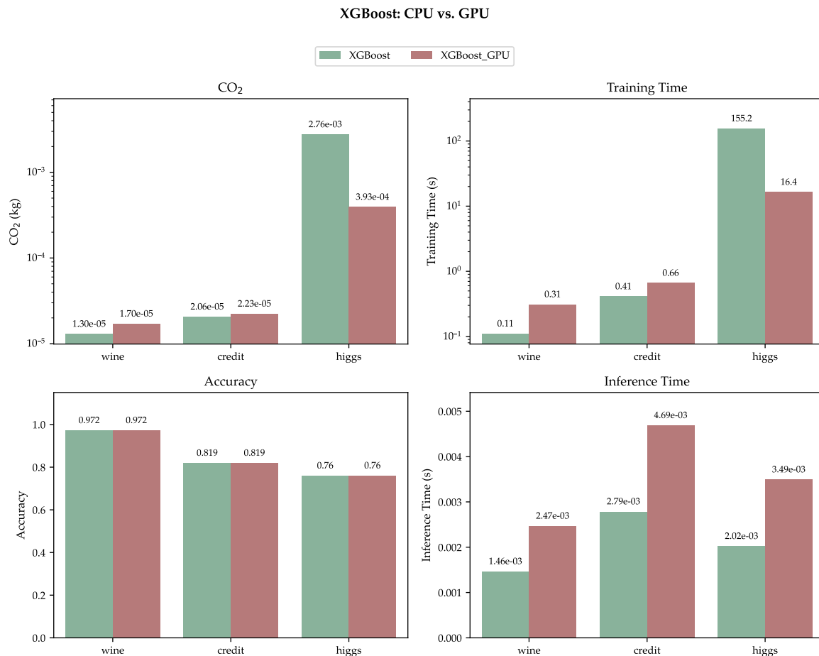
Figure 6.7: XGBoost CPU vs. GPU across datasets. Top row: CO 2 emissions and training time (log scale). Bottom row: accuracy and per-sample inference time. Accuracy is near-identical across variants on all three datasets. The ecological and speed differences are the operative comparison.
