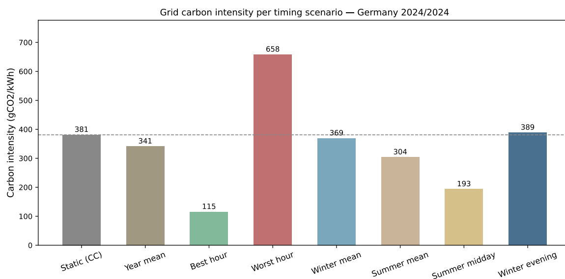
Figure 6.13: Carbon intensity (gCO 2 eq/kWh) for eight timing scenarios
