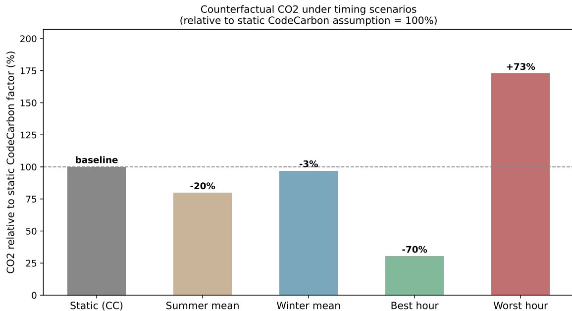
Figure 6.14: Counterfactual CO 2 relative to the static CodeCarbon baseline (= 100 %)
