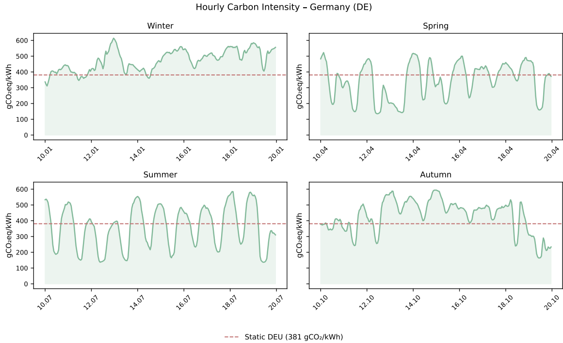
Figure 6.16: Hourly carbon intensity for representative ten-day windows per season, Germany 2025
