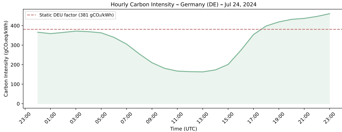
Figure 6.15: Hourly carbon intensity on 24 July 2024 in Germany
