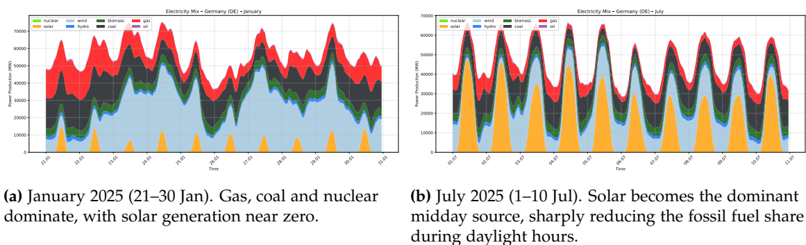
Figure 6.12: Electricity production mix in Germany for representative ten-day windows in winter and summer.
