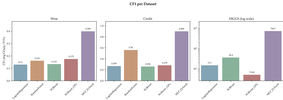
Figure 6.6: CF1 (mg CO 2 eq per WF1 percentage point) per model and dataset. Lower is better. The HIGGS panel uses a log scale. No single model leads across all three datasets.
