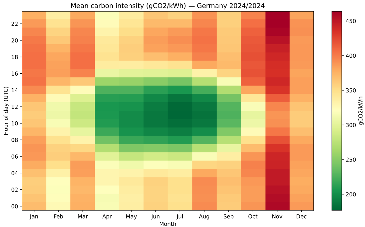
Figure 6.17: Mean carbon intensity ( \text{gCO}_2\text{eq/kWh} ) by hour of day and calendar month for the German grid (2024), derived from 8,760 hourly observations.
