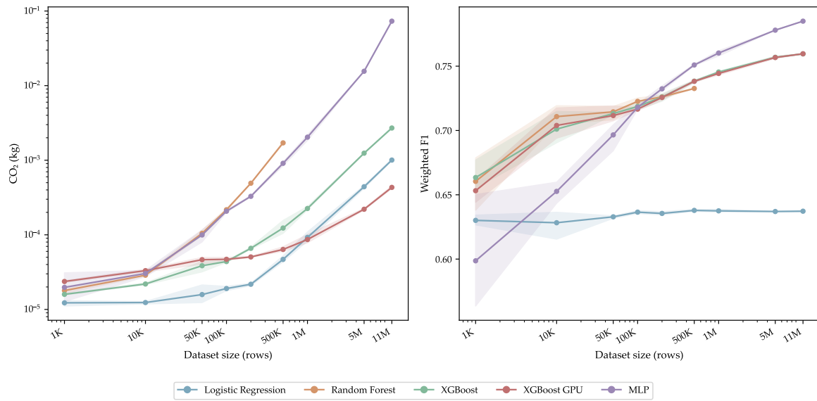
Figure 6.9: CO 2 emissions (log scale) and weighted F1-score across nine HIGGS subsets for all models. Each point is the mean of three independent random-seed runs. Random Forest excluded above 500,000 rows.
