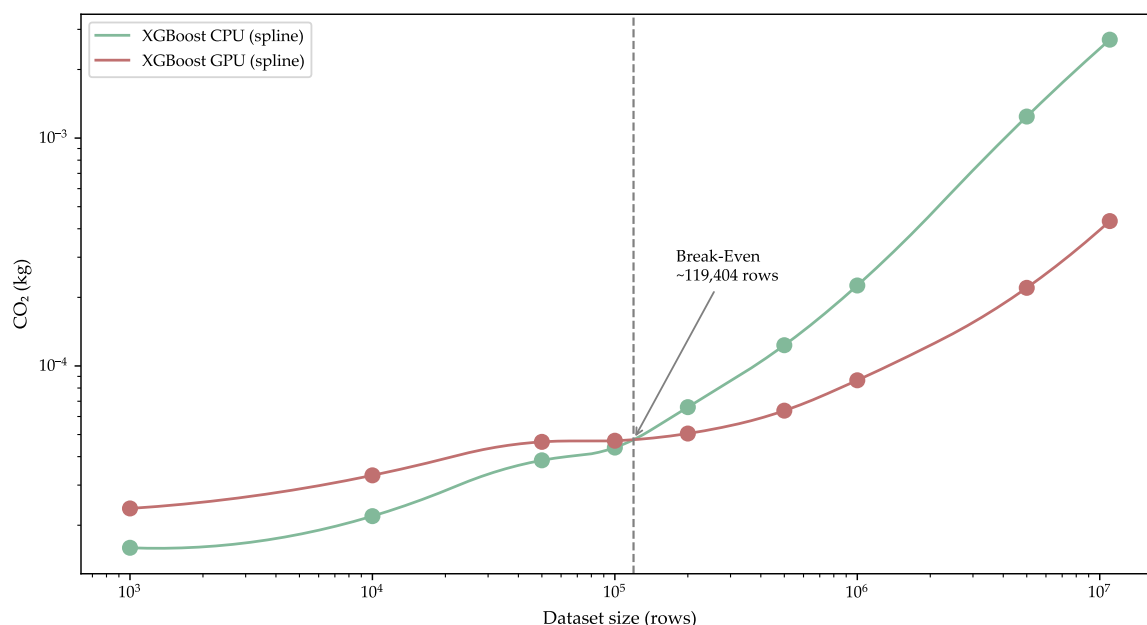
Figure 6.8: XGBoost break-even point comparison between different subset sizes of the HIGGS dataset.
