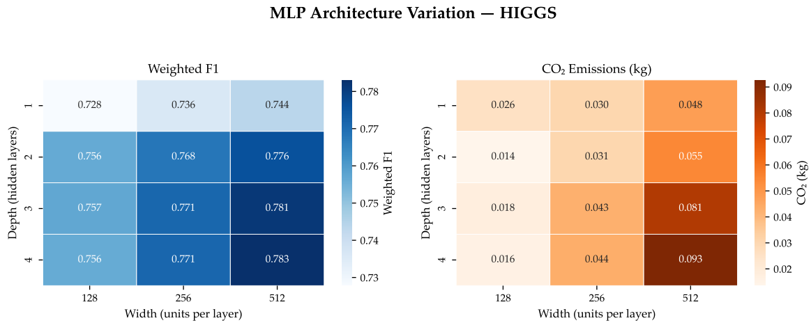
Figure 6.10: MLP architecture variation on HIGGS: weighted F1 (left) and CO 2 emissions (right) for all depth-width combinations. Darker cells indicate higher values.
