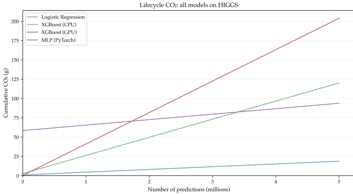
Figure 6.20: Cumulative lifecycle CO 2 for all four HIGGS models (Logistic Regression, XGBoost CPU, XGBoost GPU, MLP) as a function of prediction volume. Models with cheap training but slow inference (XGBoost GPU, XGBoost CPU) accumulate cost faster than models with expensive training but fast inference (Logistic Regression, MLP).
