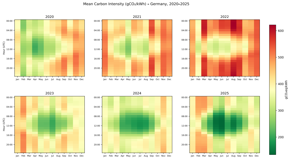
Figure 6.16: Mean carbon intensity (gCO 2 eq/kWh) by hour of day and calendar month for the German grid, 2020–2025. Each panel is derived from 8,760 hourly observations (8,784 in leap years 2020 and 2024). The shared color scale allows direct cross-year comparison. The summer-midday low-intensity band and winter-evening peak are consistent across all six years.
