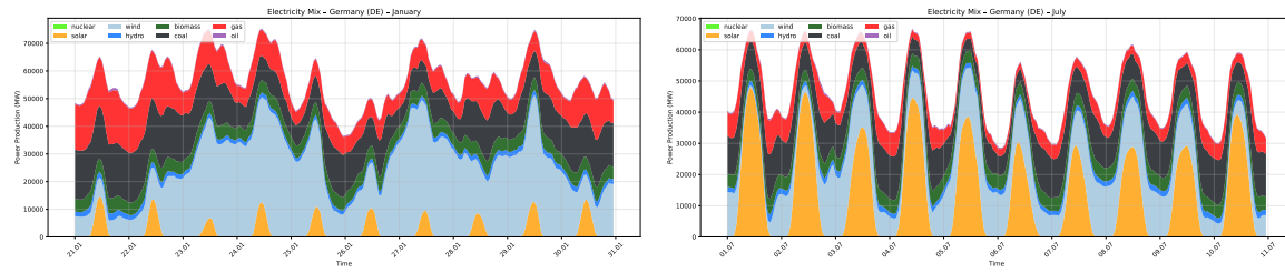
(a) January 2025 (21–30 Jan). Gas, coal and nuclear dominate, with solar generation near zero. (b) July 2025 (1–10 Jul). Solar becomes the dominant midday source, sharply reducing the fossil fuel share during daylight hours.
