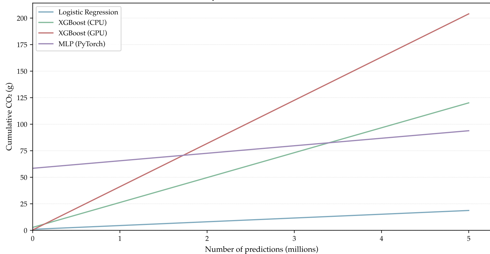
Lifecycle CO 2 : all models on HIGGS
