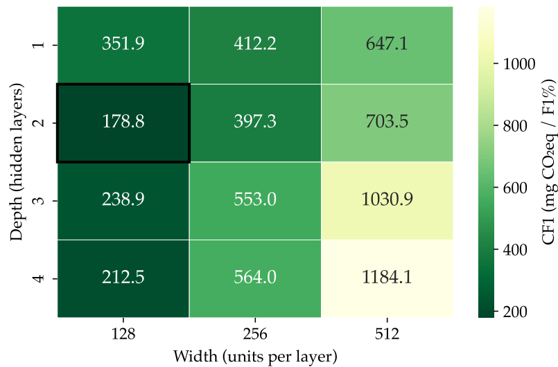
Figure 5.12: MLP architecture variation on HIGGS: CF1 for all depth-width combinations. Darker cells indicate lower (better) values.
