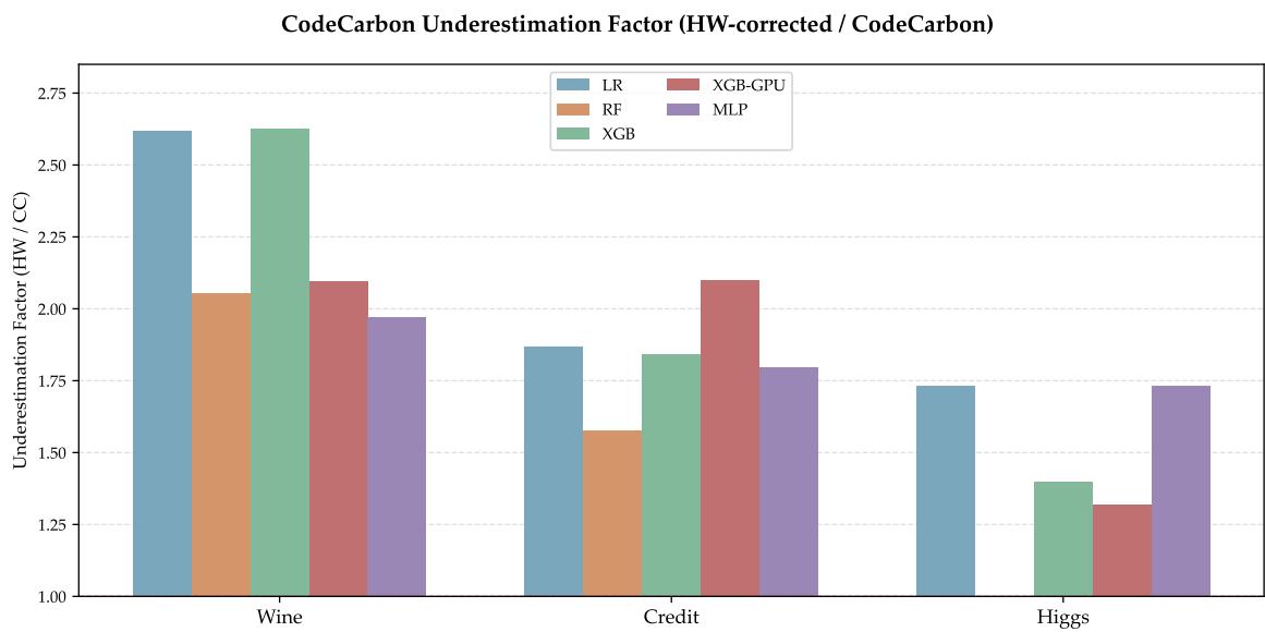
Figure 6.4: CodeCarbon underestimation factor (HW-corrected / CodeCarbon) per model and dataset. All values exceed 1, confirming systematic undercounting. Higher factors for Wine and Credit reflect CodeCarbon’s TDP-based CPU estimation being least accurate on short training runs; RF has no Higgs measurement.
