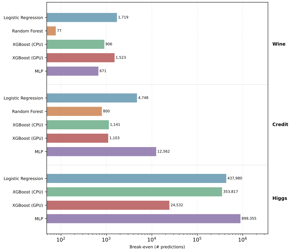
Figure 6.2: Break-even number of predictions at which cumulative inference CO 2 emissions surpass the one-time training footprint (log scale).
