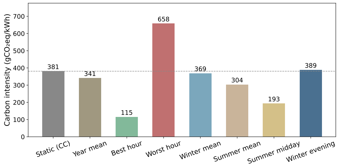
Figure 5.14: Mean grid carbon intensity in gCO 2 eq/kWh for eight timing scenarios derived from one year of hourly ElectricityMaps data for Germany (2024) [67]. The dashed line marks the static CodeCarbon baseline of 381 \frac{\text{gCO}_2\text{eq}}{\text{kWh}} . Summer midday hours are roughly half as carbon-intensive as winter evening hours, a factor of two achievable through deliberate scheduling alone.
