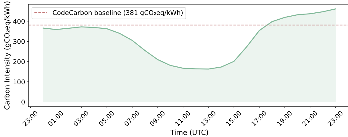
Figure 5.16: Hourly I_C in \text{gCO}_2\text{eq/kWh} for the German bidding zone on 24 July 2024, retrieved from the ElectricityMaps API [67] (/v3/carbon-intensity/past-range). Each data point represents the I_C for one clock hour as computed by ElectricityMaps from the hourly generation mix. The dashed line marks the static CodeCarbon baseline of 381 \text{ gCO}_2\text{eq/kWh} .
