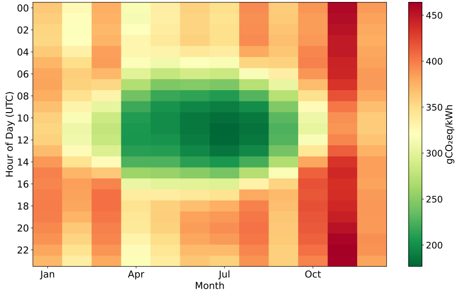
Figure 5.18: Mean carbon intensity ( \frac{\text{gCO}_2\text{eq}}{\text{kWh}} ) by hour of day and calendar month for the German grid (2024), derived from 8,760 hourly observations.
