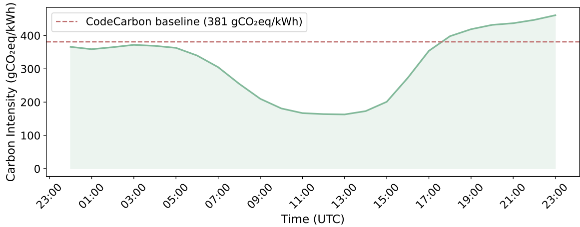
Figure 5.16: Hourly I_C in gCO 2 eq/kWh for the German bidding zone on 24 July 2024, retrieved from the ElectricityMaps API [67] (/v3/carbon-intensity/past-range). Each data point represents the I_C for one clock hour as computed by ElectricityMaps from the hourly generation mix. The dashed line marks the static CodeCarbon baseline of 381 gCO 2 eq/kWh.
