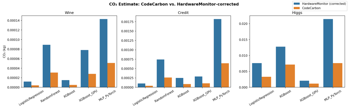
Figure 6.2: CO 2 estimate per model–dataset combination: CodeCarbon’s original total versus the sensor-corrected value used in this study.
