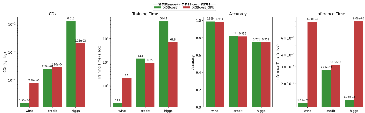
Figure 6.4: XGBoost CPU versus GPU on each dataset. From left to right: CO 2 , training time, accuracy, and inference latency.
