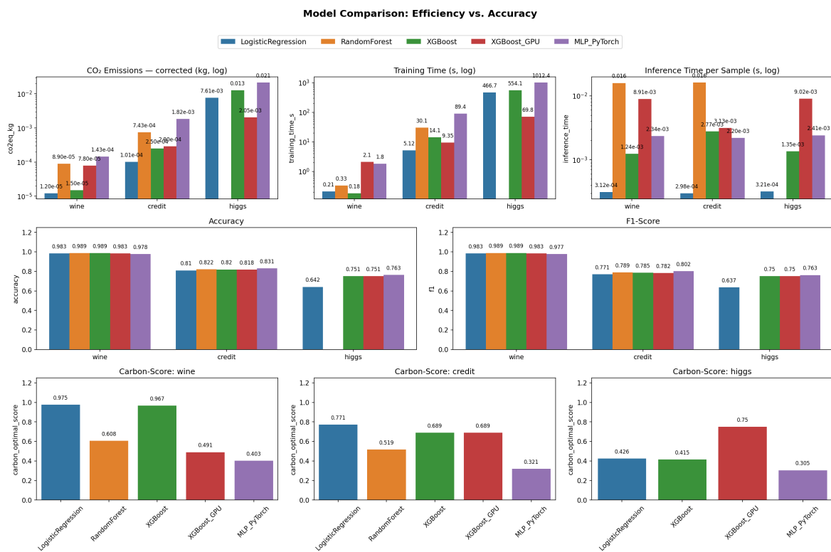
Figure 6.1: Cross-model comparison across all three datasets. Top row: training emissions, training time, and per-sample inference latency (all log-scale). Middle row: accuracy and weighted F1. Bottom row: EWF1 composite score per dataset.
