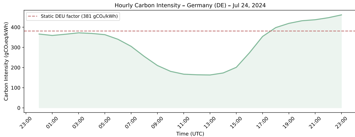
Figure 6.8: Hourly carbon intensity on 24 July 2024 in Germany
