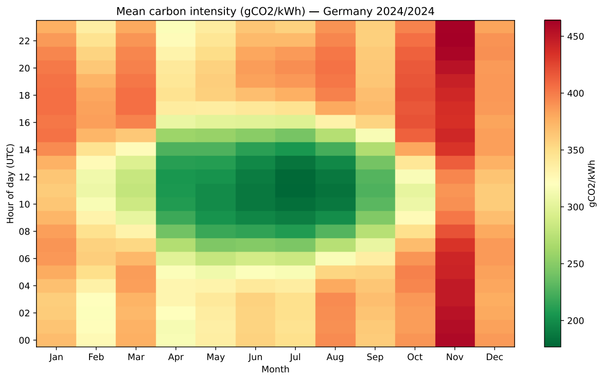
Figure 6.10: Mean carbon intensity (gCO 2 /kWh) by hour of day and calendar month for the German grid (2024), derived from 8,760 hourly observations.
