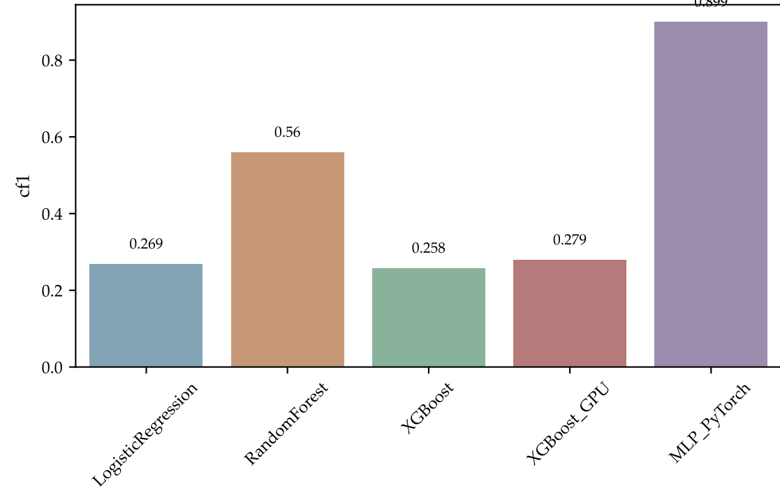
CF1: credit
