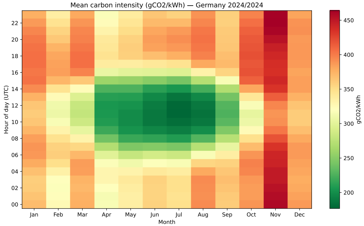
Figure 6.17: Mean carbon intensity ( \text{gCO}_2\text{eq/kWh} ) by hour of day and calendar month for the German grid (2024), derived from 8,760 hourly observations.
