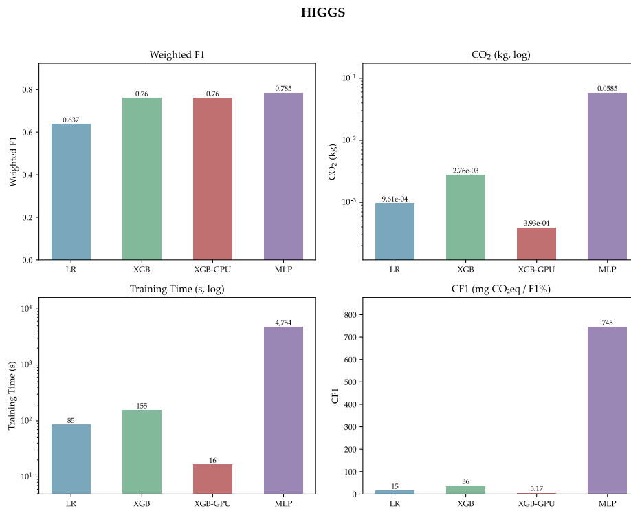
Figure C.3: Detailed benchmark results for the HIGGS dataset. Random Forest is excluded due to prohibitive training times at 11M rows.
