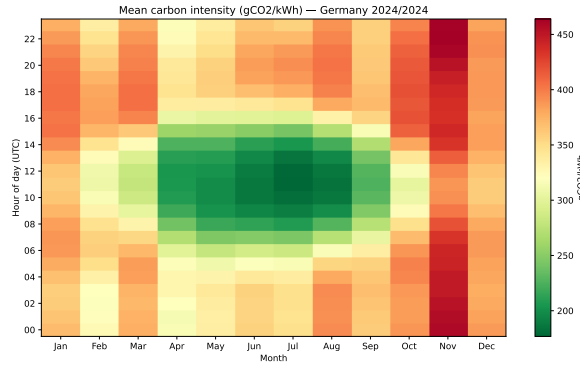
Figure 6.17: Mean carbon intensity (gCO 2 eq/kWh) by hour of day and calendar month for the German grid (2024), derived from 8,760 hourly observations.
