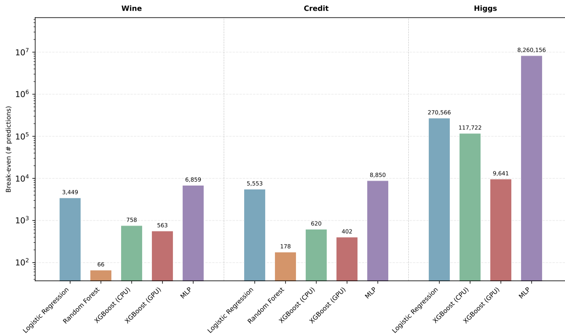
Figure 6.19: Break-even number of predictions at which cumulative inference CO 2 emissions surpass the one-time training footprint (log scale).
