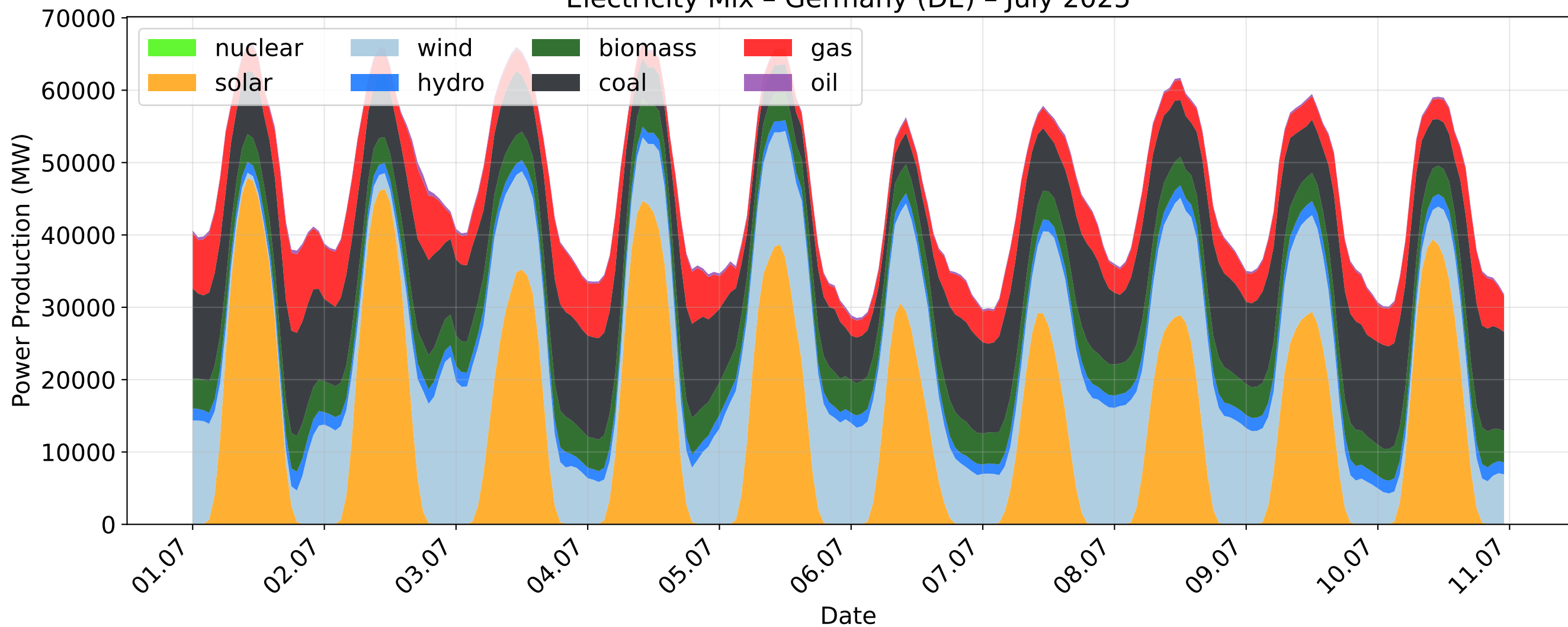
Electricity Mix - Germany (DE) - July 2025
