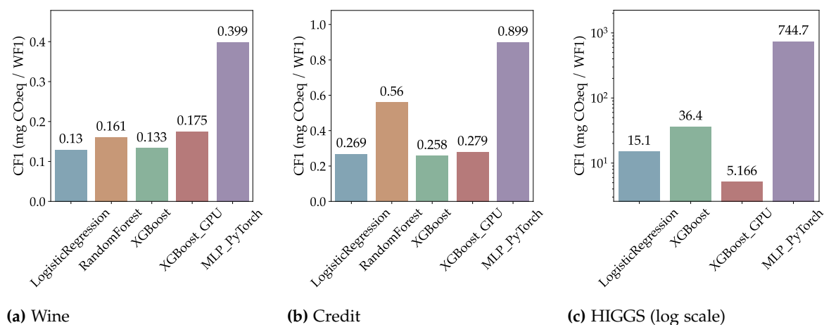
Figure 6.6: CF1 (mgCO 2 eq per WF1 percentage point) per model and dataset. Lower is better. The HIGGS panel uses a log scale. No single model leads across all three datasets.
