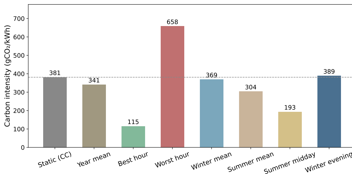
Figure 6.14: Mean grid carbon intensity in \text{gCO}_2\text{eq}/\text{kWh} for eight timing scenarios derived from one year of hourly ElectricityMaps data for Germany (2024). The dashed line marks the static CodeCarbon baseline of 381 \text{ gCO}_2\text{eq}/\text{kWh} . Summer midday hours are roughly half as carbon-intensive as winter evening hours, a factor of two achievable through deliberate scheduling alone.
