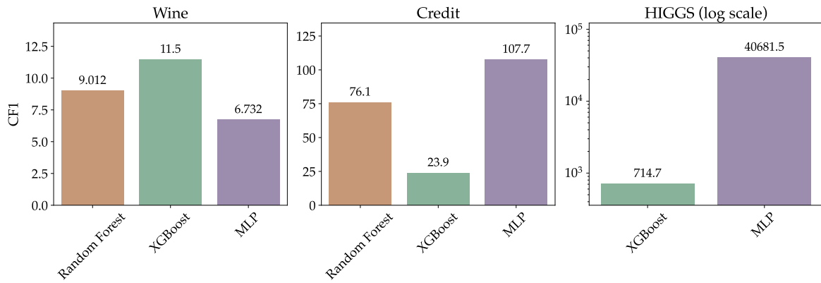
Figure 6.3: Tuning CF1 ( \frac{\text{mgCO}_2\text{eq}}{\text{WF1}} ) per tuning study, using the best WF1 across 40 trials as denominator. Lower is better. The HIGGS panel uses a log scale. RF was not tuned on HIGGS; literature defaults were used instead.
