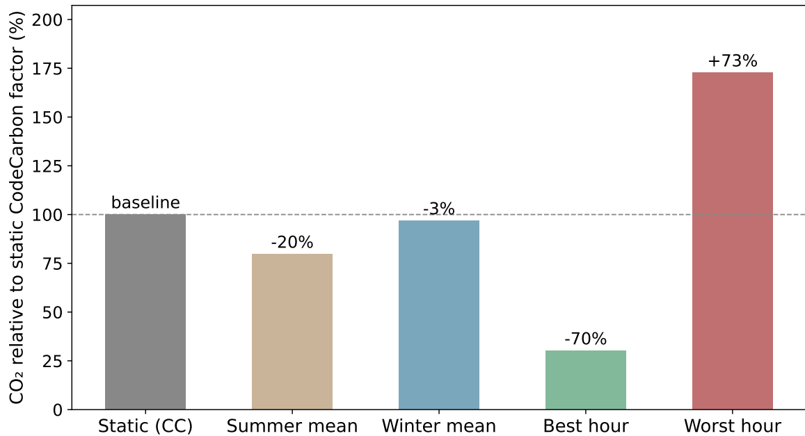
Figure 6.15: Counterfactual training emissions expressed as a percentage of the static CodeCarbon baseline (= 100 %). Because grid intensity scales uniformly across all runs, the bars are identical for every model and dataset. The dashed line marks the CodeCarbon reference; values below it represent emission reductions achievable through timing alone, without any change to code, hardware, or model architecture.
