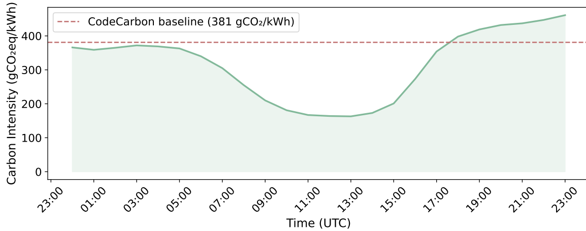
Figure 6.16: Hourly I in \text{gCO}_2\text{eq/kWh} for the German bidding zone on 24 July 2024, retrieved from the ElectricityMaps API ( /v3/carbon-intensity/past-range ). Each data point represents the I for one clock hour as computed by ElectricityMaps from the hourly generation mix. The dashed line marks the static CodeCarbon baseline of 381 \text{ gCO}_2\text{eq/kWh} .
