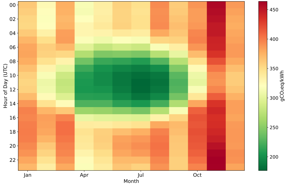
Figure 6.18: Mean carbon intensity ( \frac{gCO_2eq}{kWh} ) by hour of day and calendar month for the German grid (2024), derived from 8,760 hourly observations.
