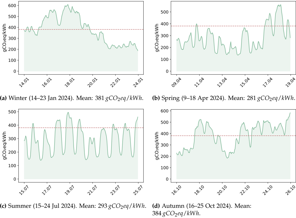
Figure 6.17: Hourly I in \text{gCO}_2\text{eq/kWh} for the German bidding zone across representative ten-day windows per season (2024), retrieved from the ElectricityMaps API ( /v3/carbon-intensity/past-range ). Each data point is the I for one clock hour. The dashed line marks the static CodeCarbon baseline of 381 \text{gCO}_2\text{eq/kWh} . Winter and autumn exceed the baseline on average; spring and summer fall below it.
