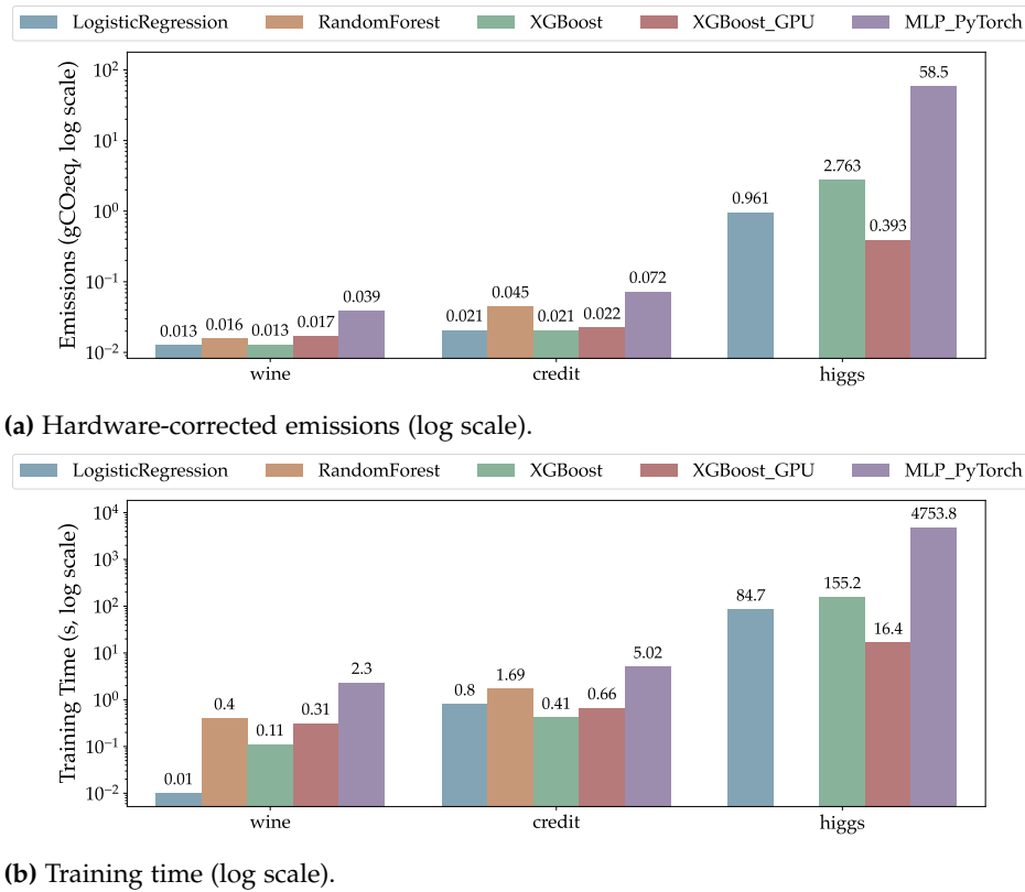
Figure 6.5: Hardware-corrected emissions and training time (log scale) across all 14 model-dataset combinations.
