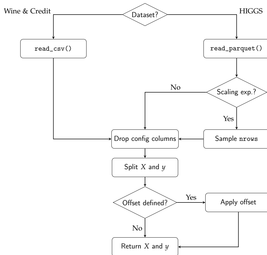
Figure 5.1: Visualization of the data loading pipeline within load_data() . The nrows sampling step only applies during the scaling experiment. The label offset ( -1 ) is applied only to the Wine dataset to shift class labels from \{1, 2, 3\} to \{0, 1, 2\} .
