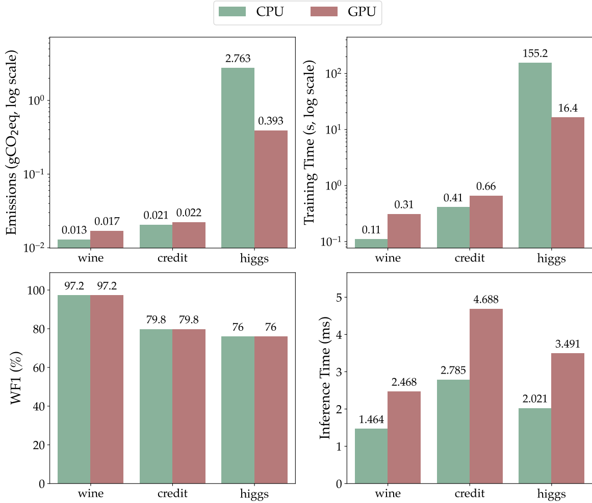
Figure 6.7: XGB CPU vs. GPU across datasets. Top row: Emissions in gCO 2 eq and training time in seconds (log scale). Bottom row: WF1 and per-sample inference time. WF1 is identical across variants on all three datasets. The ecological and speed differences are the operative comparison.
