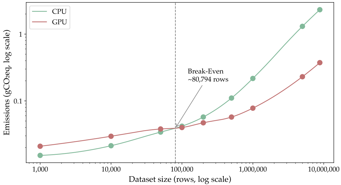
Figure 6.8: XGB break-even point comparison between different subset sizes of the HIGGS dataset.
