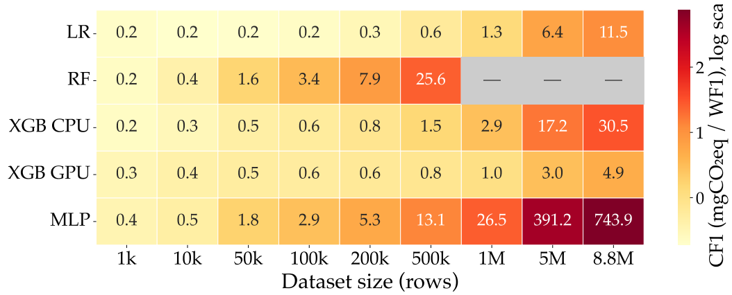
Figure 6.10: CF1 (mgCO 2 eq per WF1) for all model-size combinations. Colour encodes log-scaled CF1: yellow is most efficient, dark red is least. Cell annotations show raw CF1 values. Grey cells indicate runs not performed (RF excluded above 500,000 rows).
