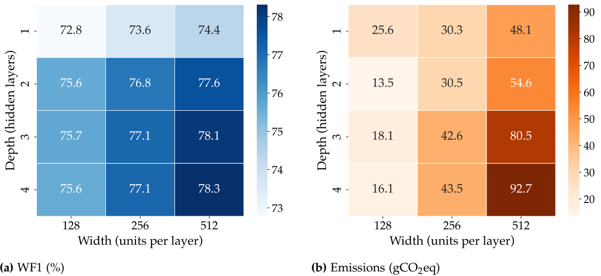
Figure 6.11: MLP architecture variation on HIGGS for all depth-width combinations. Left: WF1, where darker cells indicate higher WF1 (better). Right: training emissions in gCO 2 eq, where lighter cells indicate lower emissions (better).
