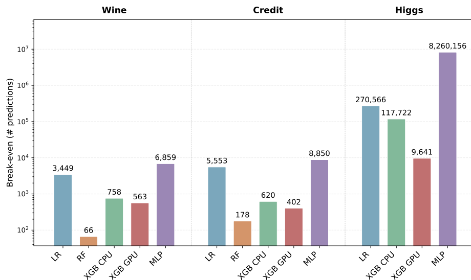
Figure 6.20: Break-even number of predictions at which cumulative inference emissions surpass the one-time training footprint (log scale).
