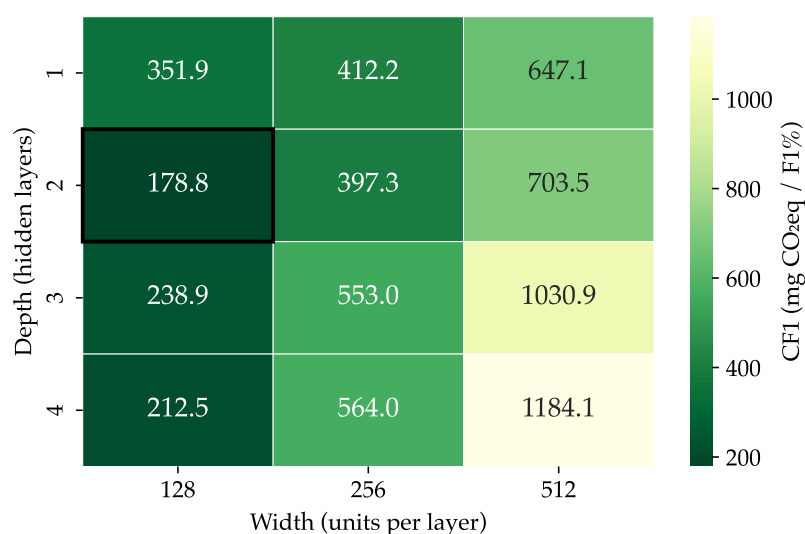
Figure 6.12: MLP architecture variation on HIGGS: CF1 for all depth-width combinations. Darker cells indicate lower (better) values.
