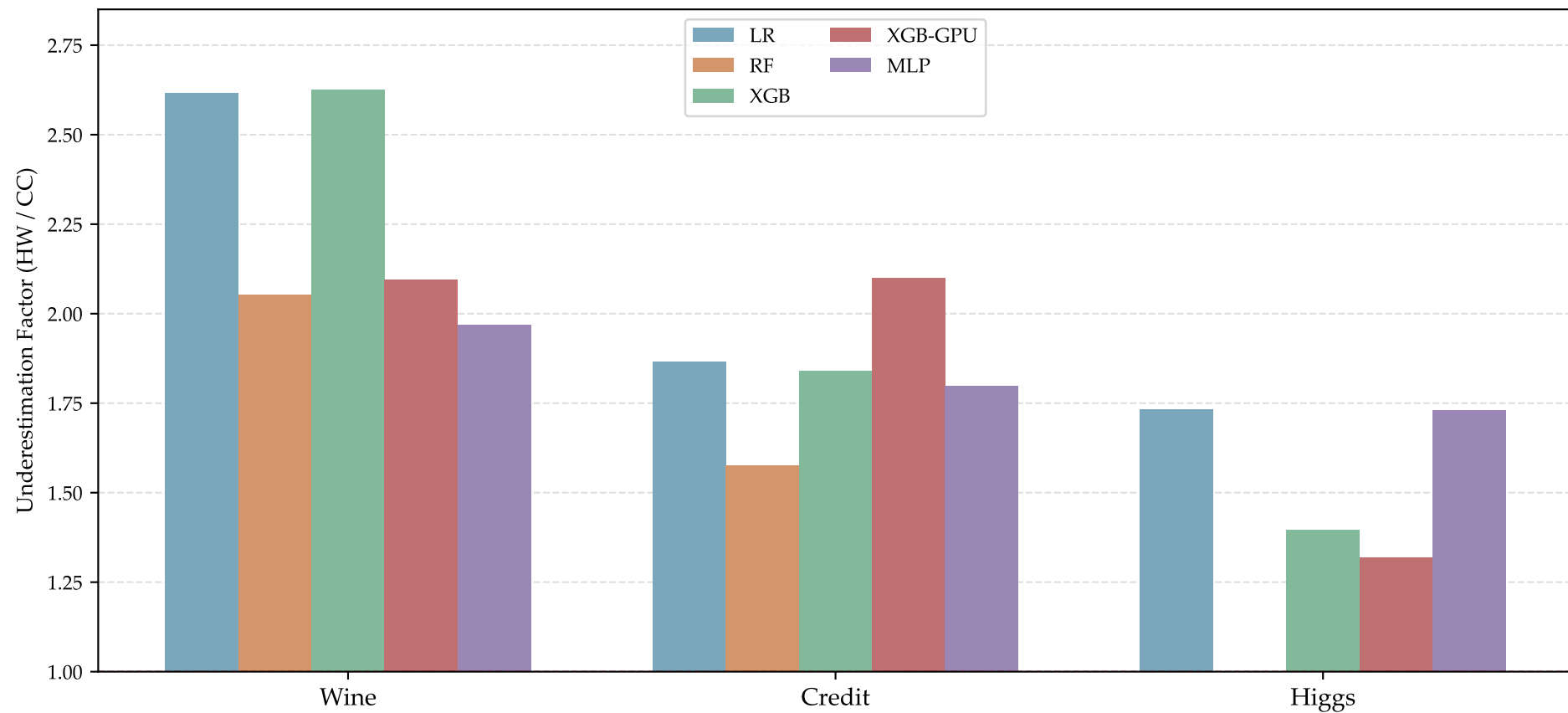
CodeCarbon Underestimation Factor (HW-corrected / CodeCarbon)
