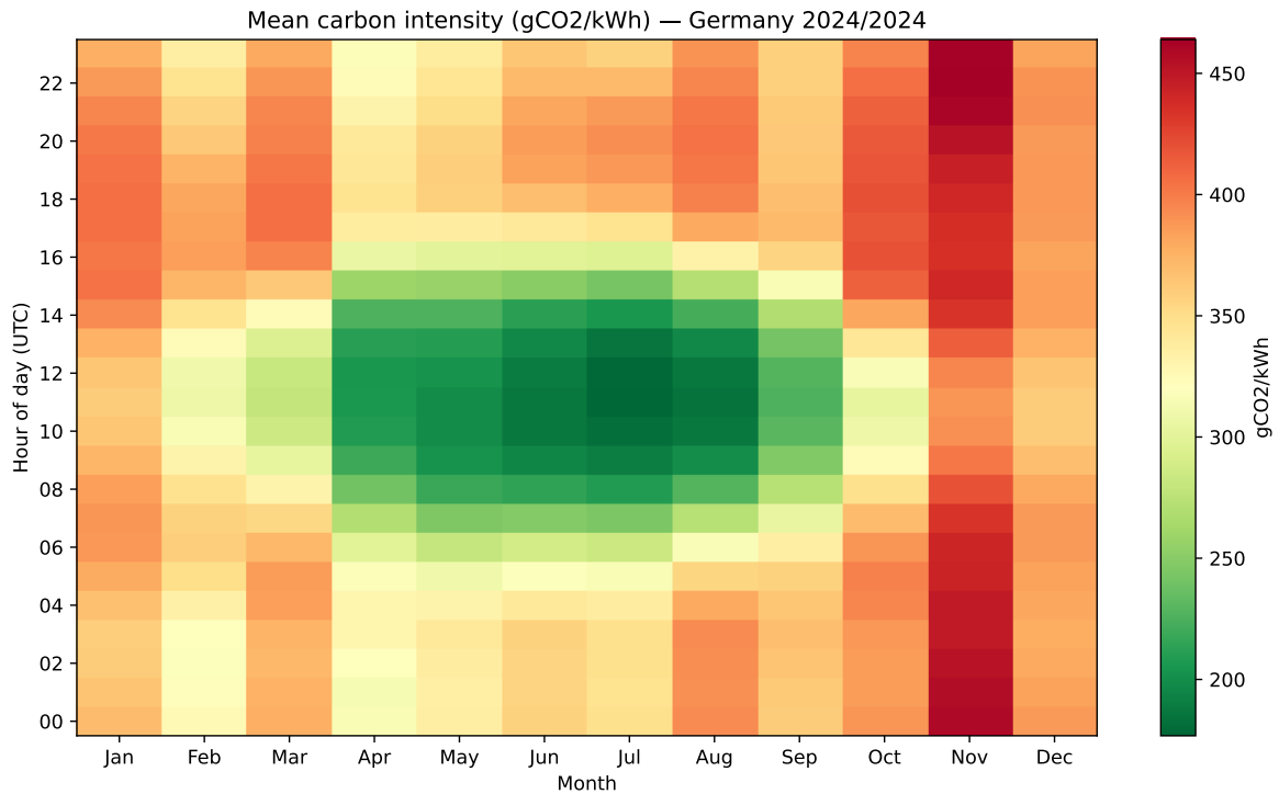
Figure 6.11: Mean carbon intensity ( \text{gCO}_2/\text{kWh} ) by hour of day and calendar month for the German grid (2024), derived from 8,760 hourly observations.
