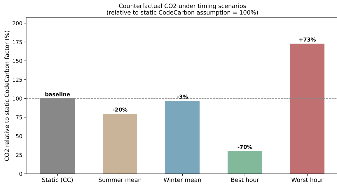
Figure 6.8: Counterfactual CO 2 relative to the static CodeCarbon baseline (= 100 %)
