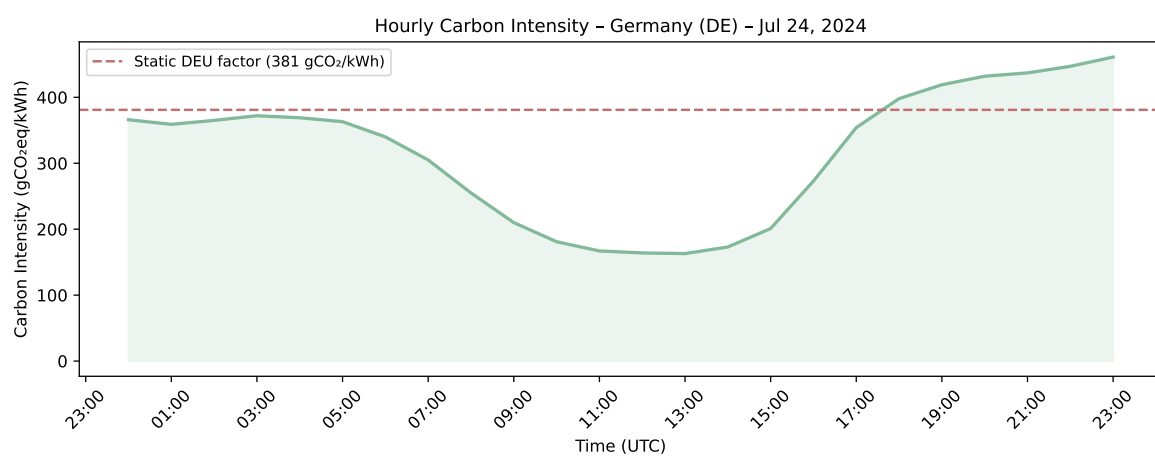
Figure 6.9: Hourly carbon intensity on 24 July 2024 in Germany
