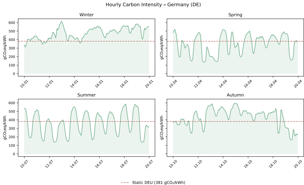
Figure 6.10: Hourly carbon intensity for representative ten-day windows per season, Germany 2025
