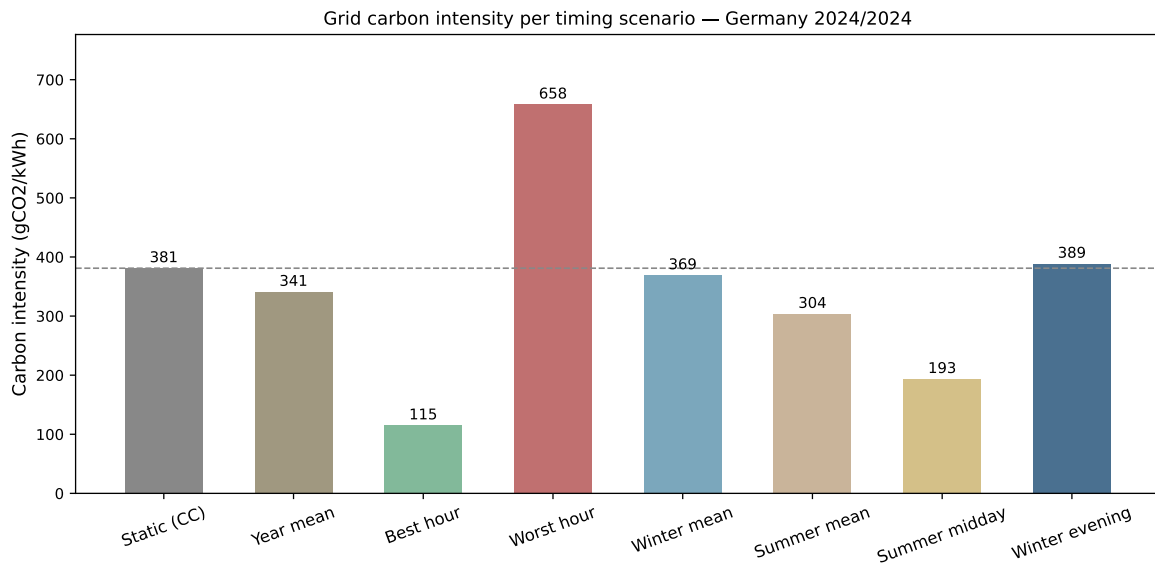
Figure 6.7: Carbon intensity (gCO 2 /kWh) for eight timing scenarios
