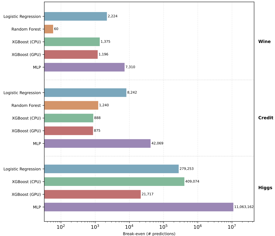
Figure 6.12: Break-even number of predictions at which cumulative inference CO 2 emissions surpass the one-time training footprint (log scale).
