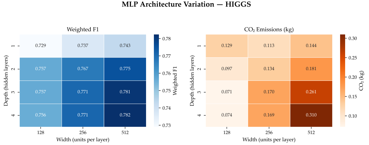
Figure 6.6: MLP architecture variation on HIGGS: weighted F1 (left) and CO 2 emissions (right) for all depth-width combinations. Darker cells indicate higher values.
