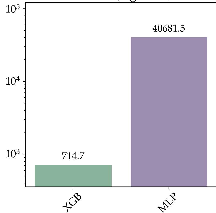
HIGGS (log scale)
