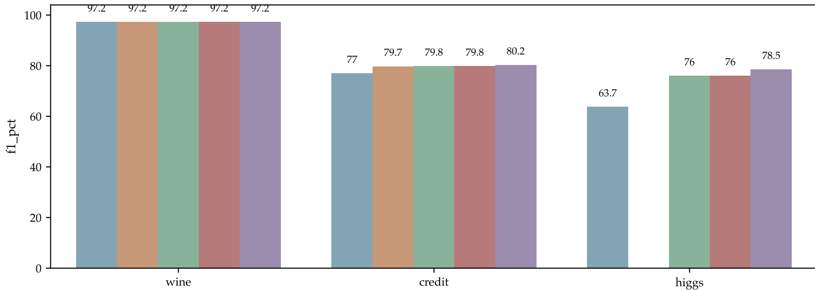
CF1: credit
