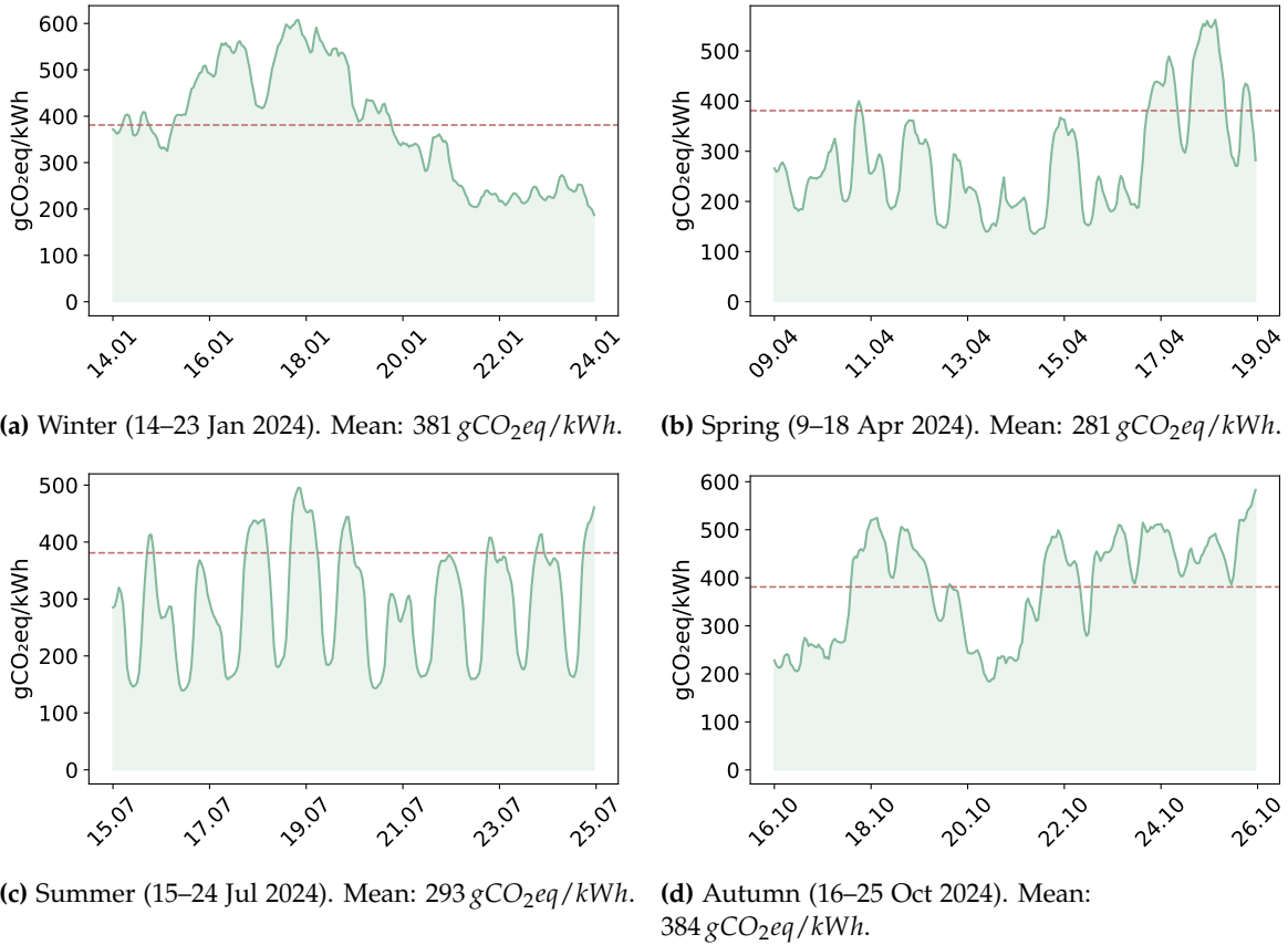
Figure 5.17: Hourly I_C in \text{gCO}_2\text{eq/kWh} for the German bidding zone across representative ten-day windows per season (2024), retrieved from the ElectricityMaps API ( /v3/carbon-intensity/past-range ). Each data point is the I_C for one clock hour. The dashed line marks the static CodeCarbon baseline of 381 \text{gCO}_2\text{eq/kWh} . Winter and autumn exceed the baseline on average; spring and summer fall below it.
